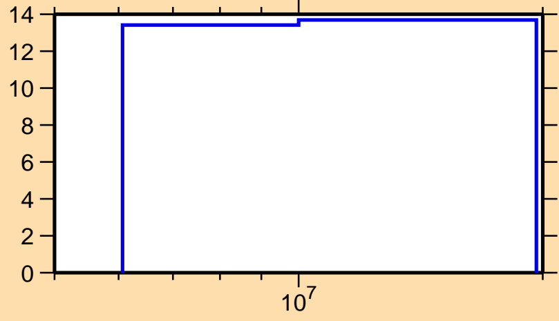
\Delta\sigma/\sigma vs. E for ^{47}\text{K}(n,n\text{onel.})
