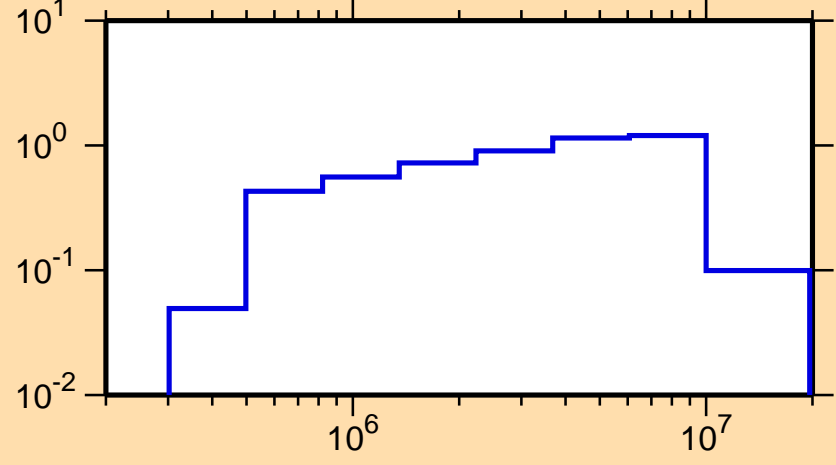
\sigma vs. E for ^{47}\text{K}(n,\text{inel.})
