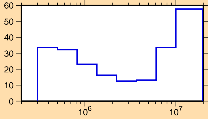
\Delta\sigma/\sigma vs. E for ^{47}\text{K}(n,\text{inel.})
