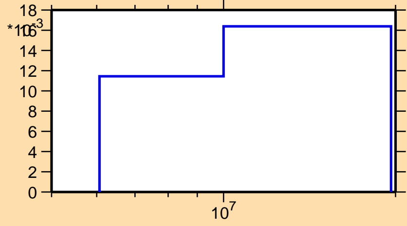
\sigma vs. E for ^{47}\text{K}(n,n\text{cont.})
