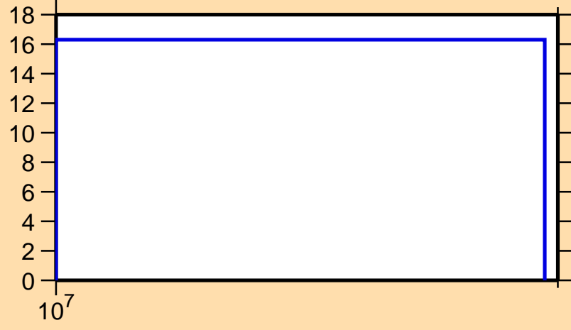
\Delta\sigma/\sigma vs. E for ^{47}\text{K}(n,2n)
