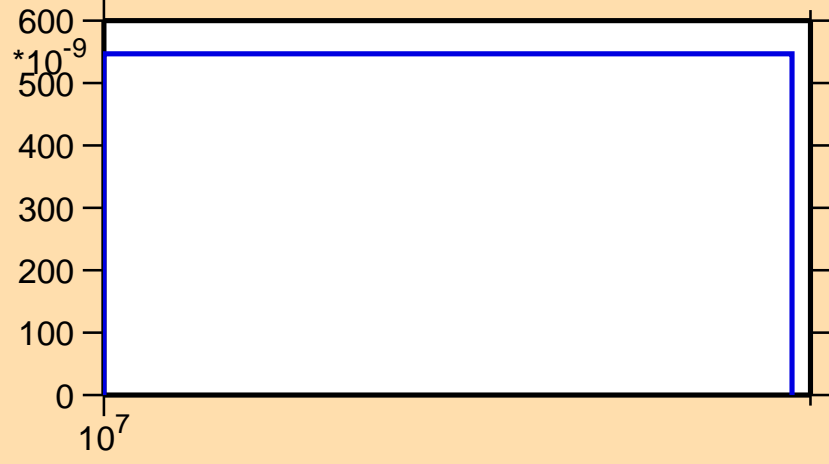
\sigma vs. E for ^{47}\text{K}(n,np)
