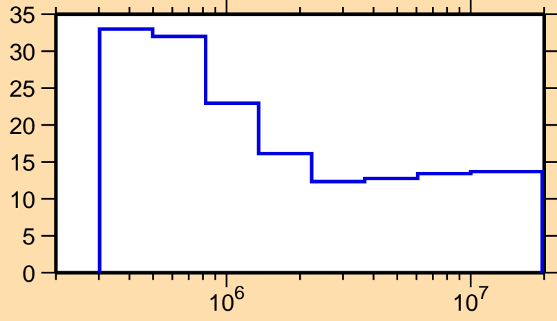
\Delta\sigma/\sigma vs. E for ^{47}\text{K}(n,\text{nonel.})
