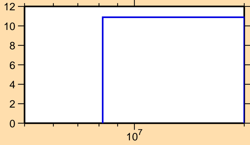
\Delta\sigma/\sigma vs. E for ^{47}\text{K}(n,el.)
