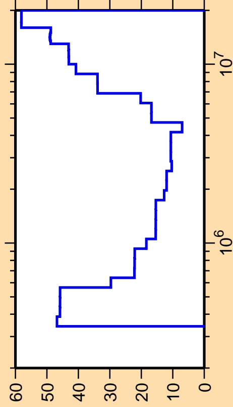
\Delta\sigma/\sigma vs. E for ^{48}\text{K}(n,\text{inel.})
