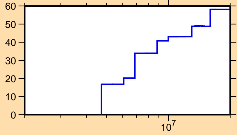
\Delta\sigma/\sigma vs. E for ^{48}\text{K}(n,\text{inel.})
