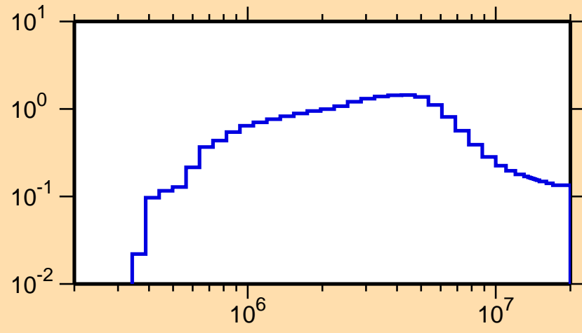
\sigma vs. E for ^{48}\text{K}(n,\text{inel.})
