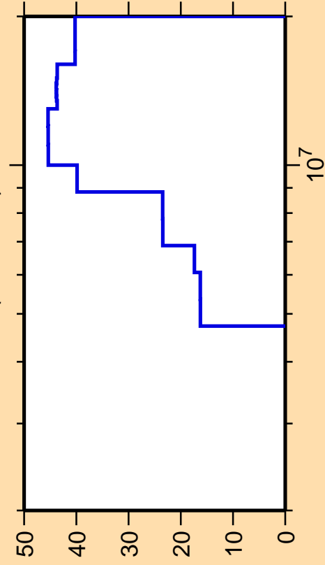
\Delta\sigma/\sigma vs. E for ^{48}\text{K}(n,n\text{cont.})
