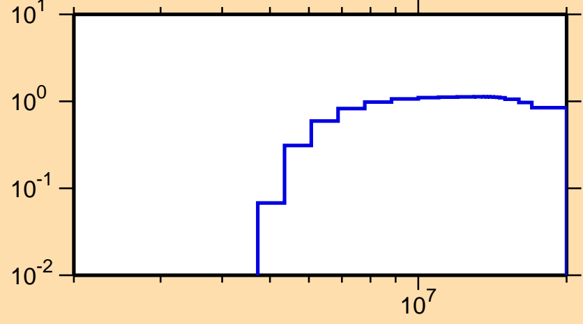
\sigma vs. E for ^{48}\text{K}(n,2n)
