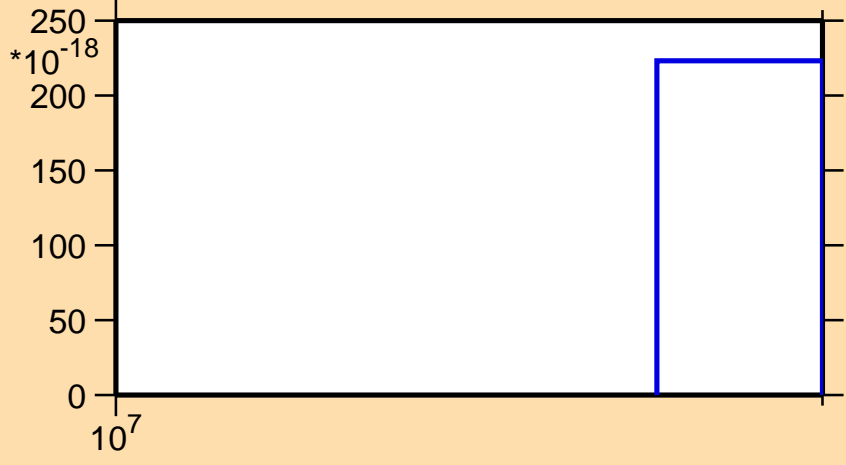
\sigma vs. E for ^{48}\text{K}(n,2n\alpha)
