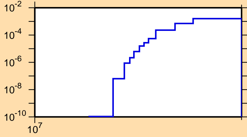
\sigma vs. E for ^{48}\text{K}(n,d)
