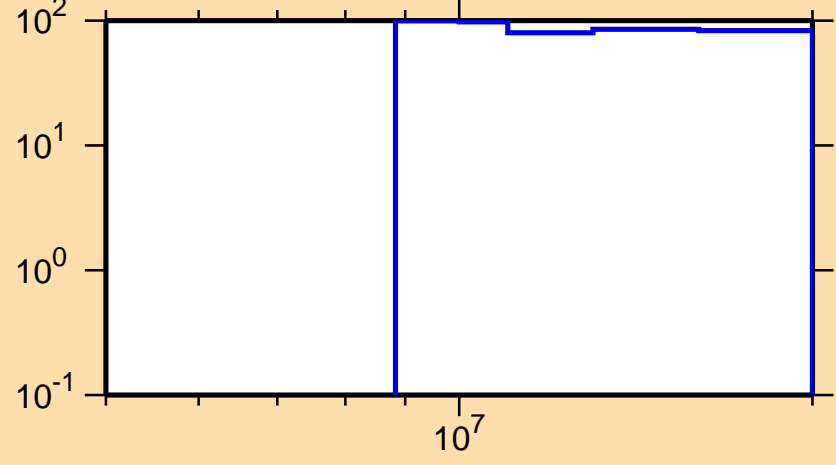
\Delta\sigma/\sigma vs. E for ^{48}\text{K}(n,p)
