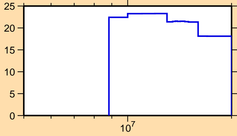
\Delta\sigma/\sigma vs. E for ^{48}\text{K}(n,el.)
