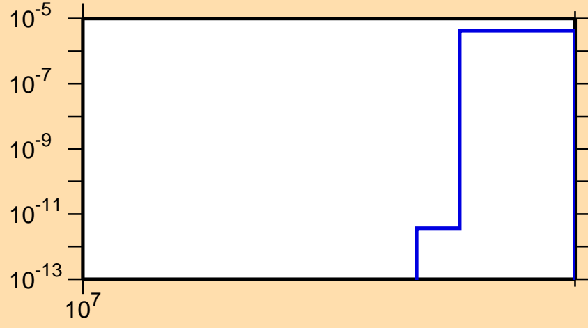
\sigma vs. E for ^{48}\text{K}(n,nd)
