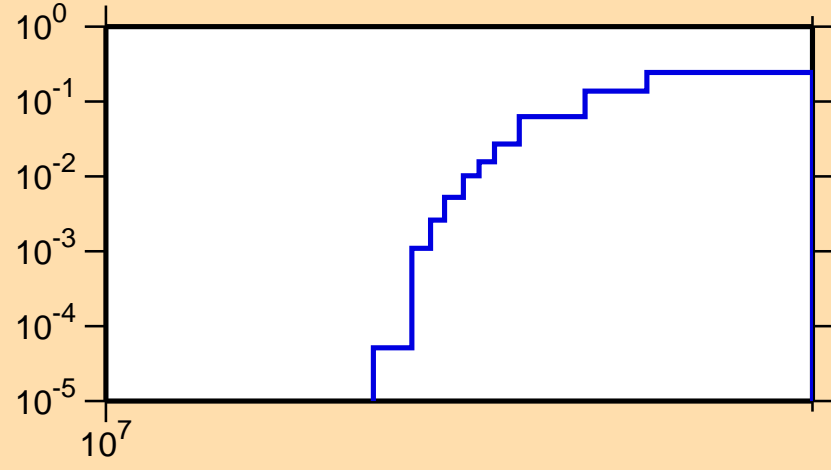
\sigma vs. E for ^{48}\text{K}(n,3n)
