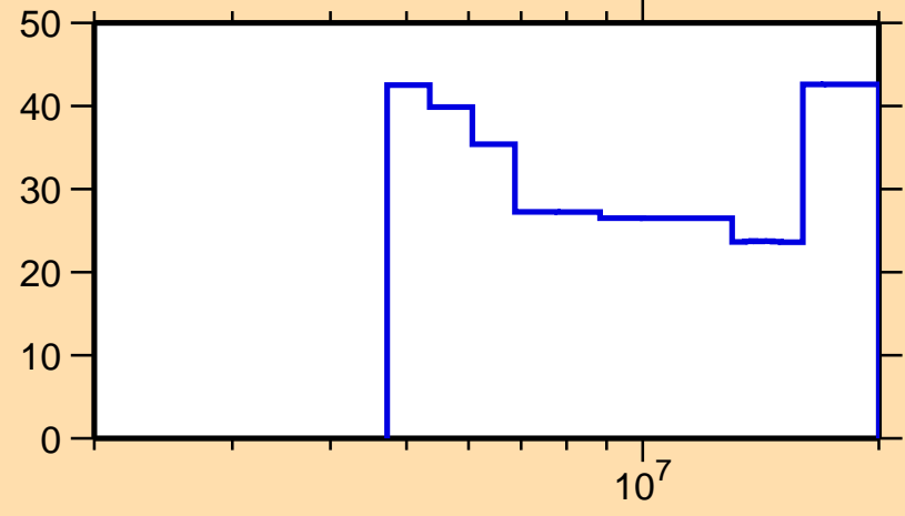
\Delta\sigma/\sigma vs. E for ^{48}\text{K}(n,2n)
