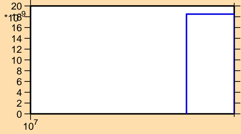
\sigma vs. E for ^{48}\text{K}(n,nt)
