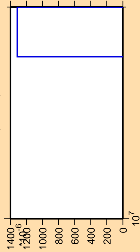
\Delta\sigma/\sigma vs. E for ^{48}\text{K}(n,2n\alpha)
