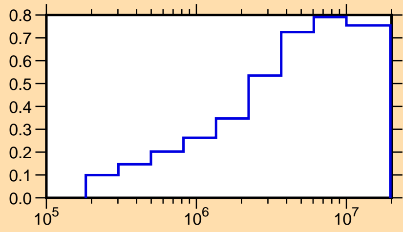
\mu vs. E for ^{48}\text{K}(\text{mt251})
