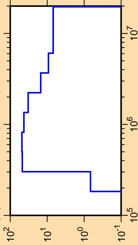
\Delta\mu/\mu vs. E for ^{48}\text{K}(\text{mt251})
