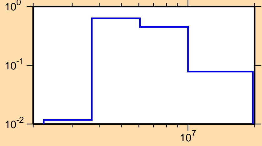
\sigma vs. E for ^{48}\text{K}(n,n\text{cont.})
