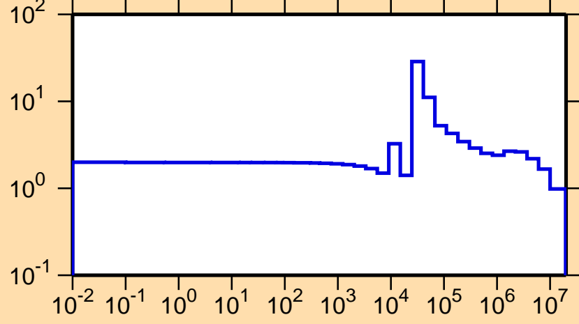
\sigma vs. E for ^{48}\text{K}(n,\text{el.})
