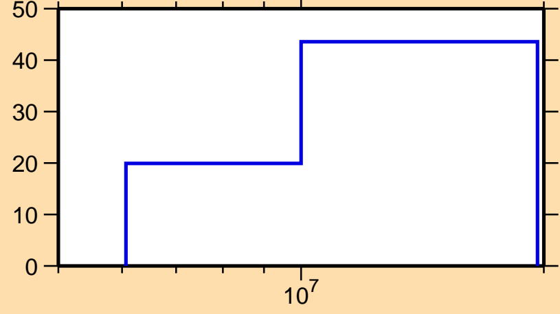
\Delta\sigma/\sigma vs. E for ^{48}\text{K}(n,ncont.)
