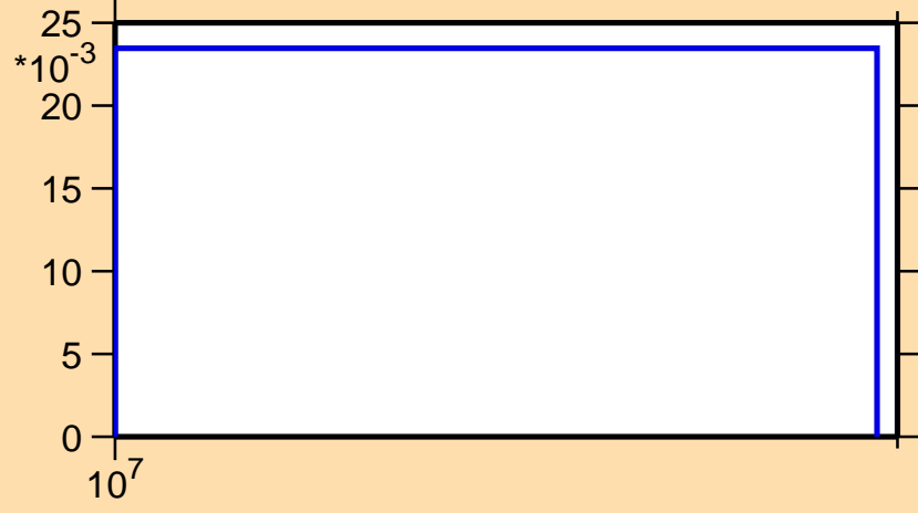
\sigma vs. E for ^{48}\text{K}(n,3n)
