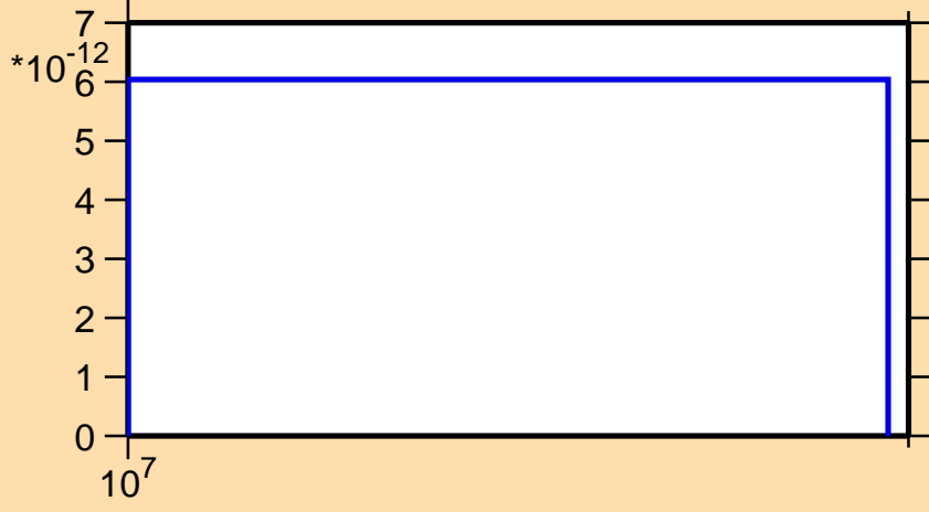
\sigma vs. E for ^{48}\text{K}(n,2np)
