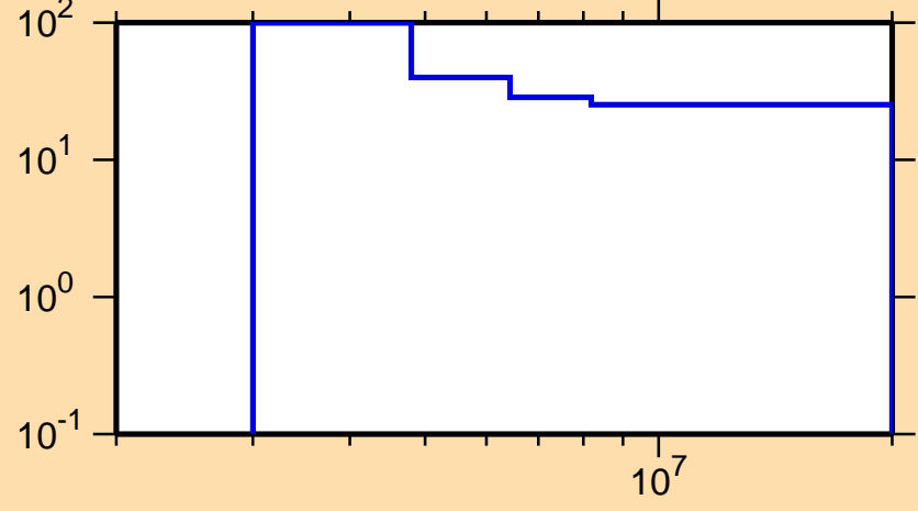
\Delta\sigma/\sigma vs. E for ^{48}\text{K}(n,2n)
