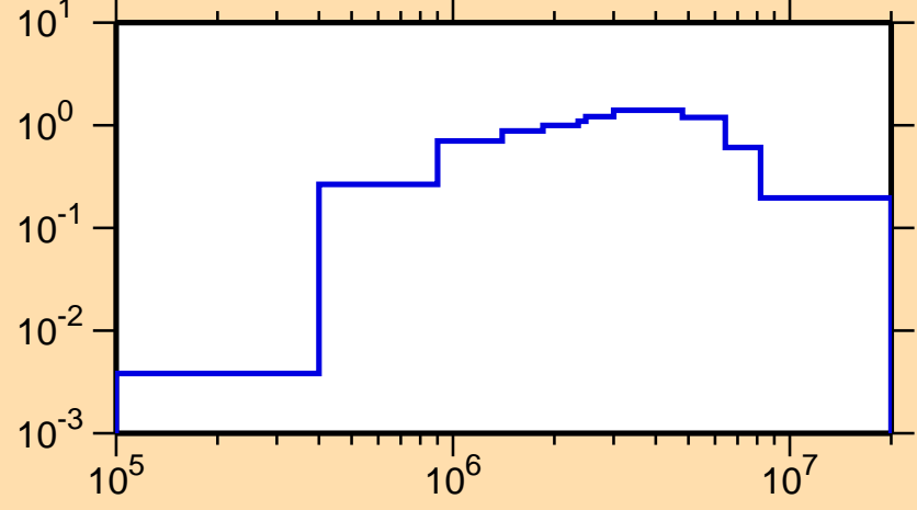
\sigma vs. E for ^{48}\text{K}(n,\text{inel.})
