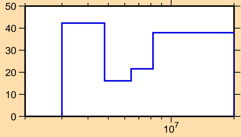
\Delta\sigma/\sigma vs. E for ^{48}\text{K}(n,n\text{cont.})
