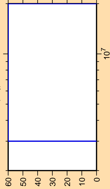
\Delta\sigma/\sigma vs. E for ^{48}\text{K}(n,\gamma)
