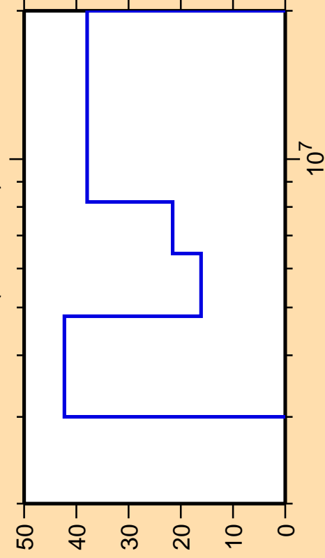
\Delta\sigma/\sigma vs. E for ^{48}\text{K}(n,ncont.)
