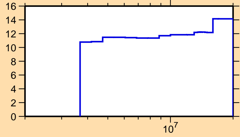
\Delta\sigma/\sigma vs. E for ^{49}\text{K}(n,n\text{onel.})
