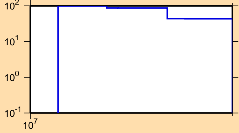
\Delta\sigma/\sigma vs. E for ^{49}\text{K}(n,p)
