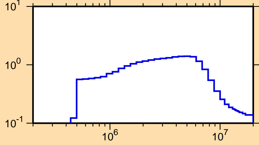
\sigma vs. E for ^{49}\text{K}(n,\text{inel.})
