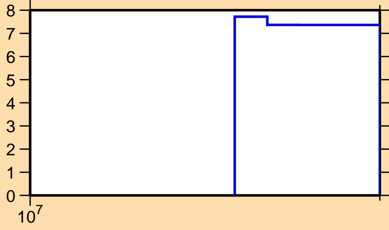
\Delta\sigma/\sigma vs. E for ^{72}\text{Kr}(n,el.)
