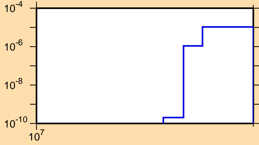
\sigma vs. E for ^{72}\text{Kr}(n,2n)
