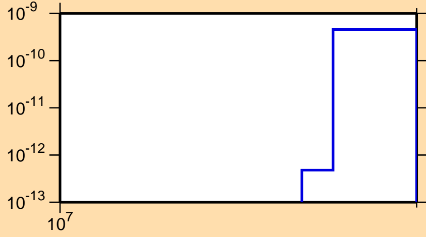
\sigma vs. E for ^{72}\text{Kr}(\text{mt } 34)
