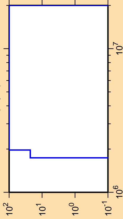
\Delta\sigma/\sigma vs. E for ^{72}\text{Kr}(n,p\alpha)
