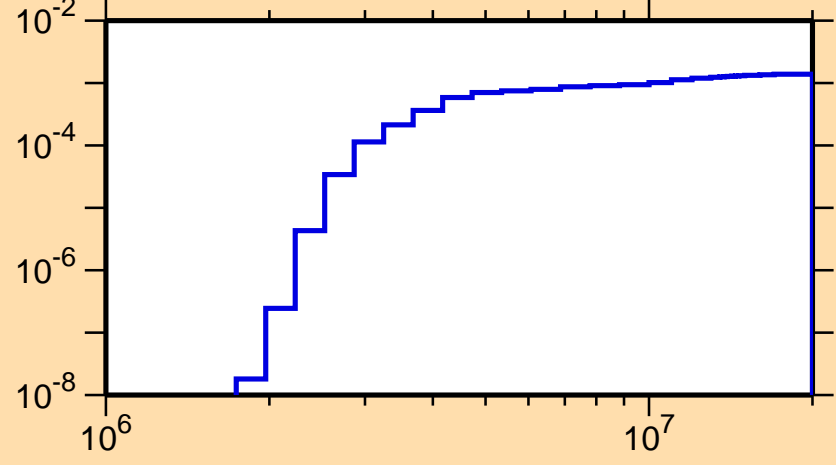
\sigma vs. E for ^{72}\text{Kr}(n,n\text{cont.})
