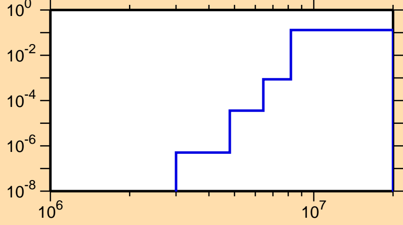
\sigma vs. E for ^{72}\text{Kr}(n,p\alpha)
