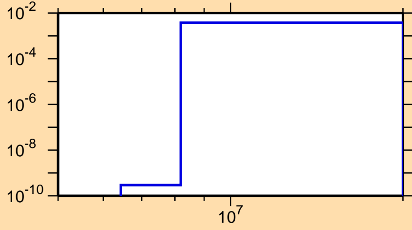
\sigma vs. E for ^{72}\text{Kr}(n,\text{pd})
