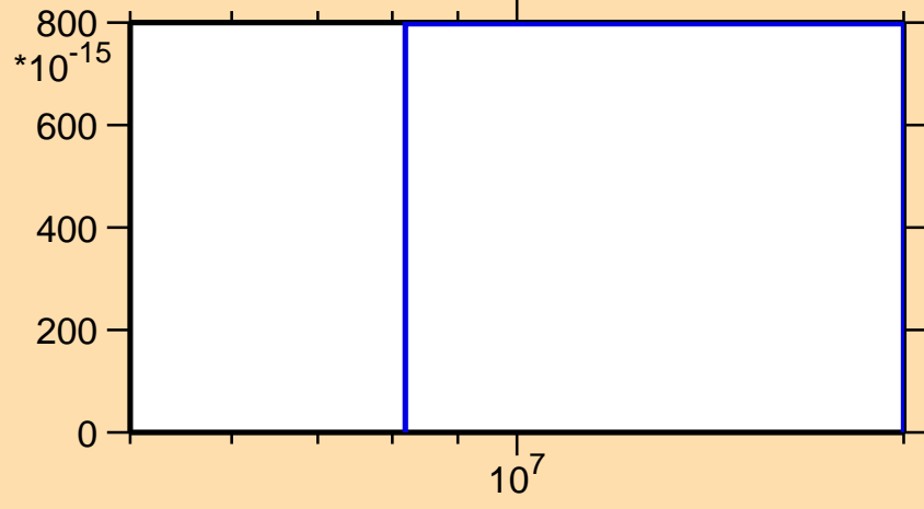
\sigma vs. E for ^{72}\text{Kr}(n,\text{nd})
