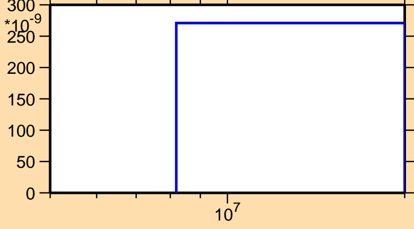
\sigma vs. E for ^{72}\text{Kr}(n,pt)
