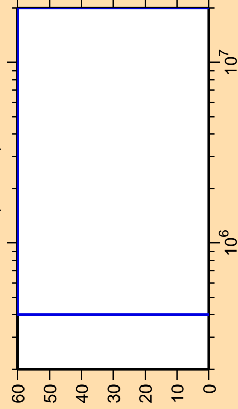
\Delta\sigma/\sigma vs. E for ^{72}\text{Kr}(n,\text{inel.})
