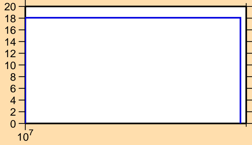
\Delta\sigma/\sigma vs. E for ^{73}\text{Kr}(n,el.)
