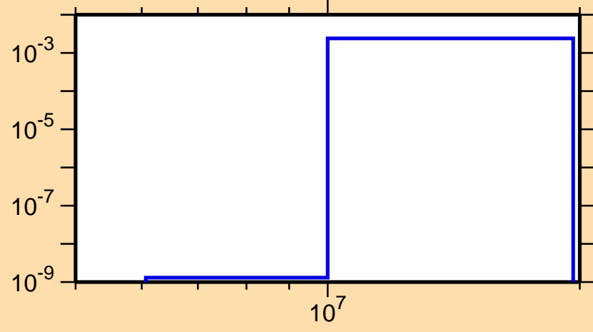
\sigma vs. E for ^{73}\text{Kr}(n,pd)
