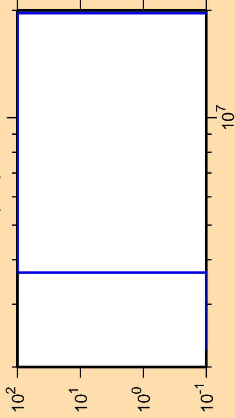
\Delta\sigma/\sigma vs. E for ^{73}\text{Kr}(n,d)
