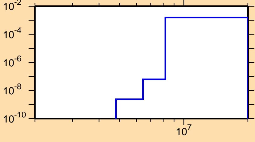
\sigma vs. E for ^{73}\text{Kr}(n,\text{He3})
