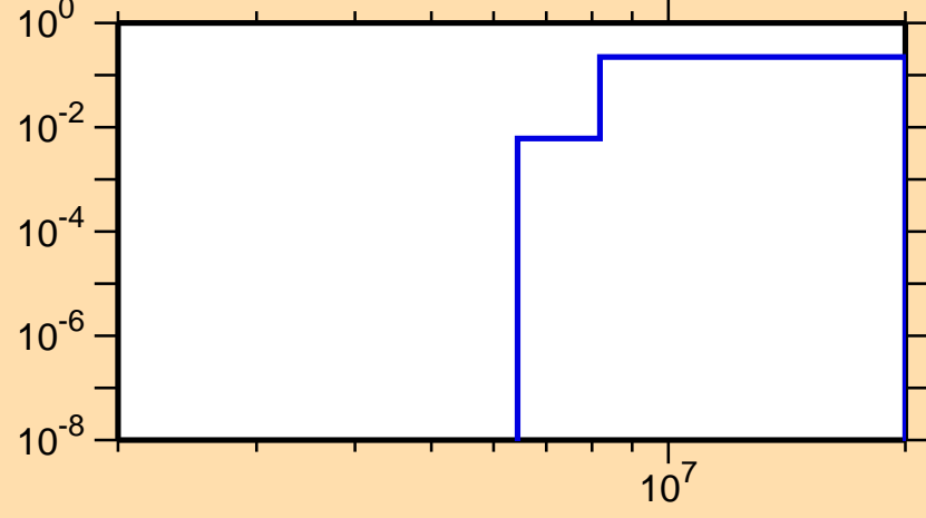
\sigma vs. E for ^{73}\text{Kr}(n,np)
