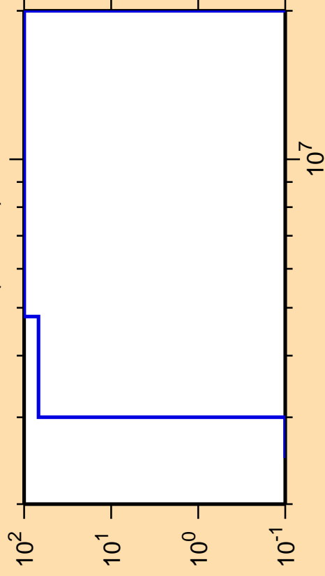
\Delta\sigma/\sigma vs. E for ^{73}\text{Kr}(n,\text{He3})
