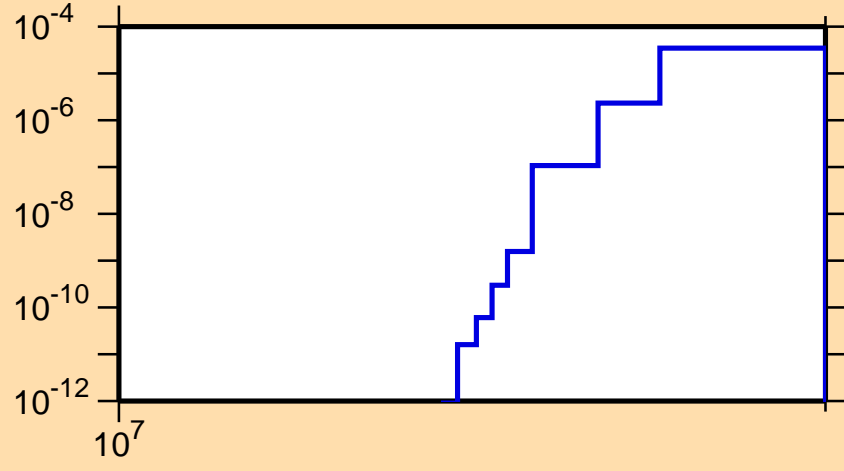
\sigma vs. E for ^{75}\text{Kr}(n,pt)
