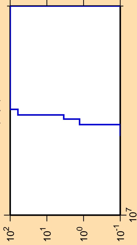
\Delta\sigma/\sigma vs. E for ^{75}\text{Kr}(n,pt)
