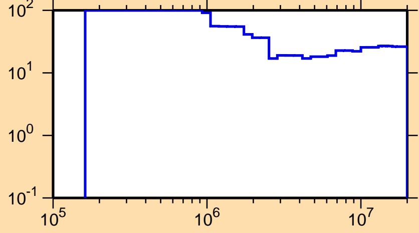
\Delta\sigma/\sigma vs. E for ^{75}\text{Kr}(n,\text{inel.})
