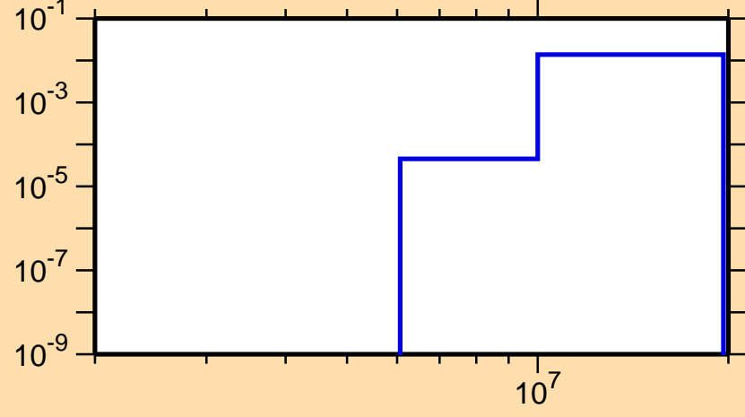
\sigma vs. E for ^{75}\text{Kr}(n,d)
