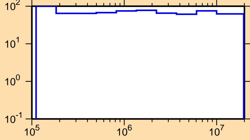
\Delta\sigma/\sigma vs. E for ^{75}\text{Kr}(n,n_1)
