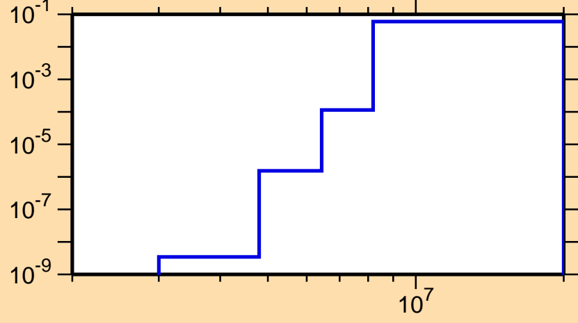
\sigma vs. E for ^{75}\text{Kr}(n,p\alpha)
