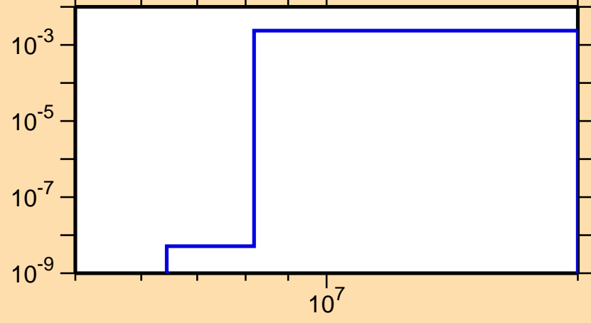
\sigma vs. E for ^{75}\text{Kr}(n,\alpha)
