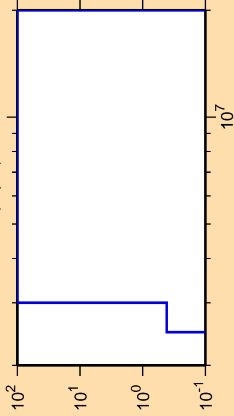
\Delta\sigma/\sigma vs. E for ^{75}\text{Kr}(n,p\alpha)
