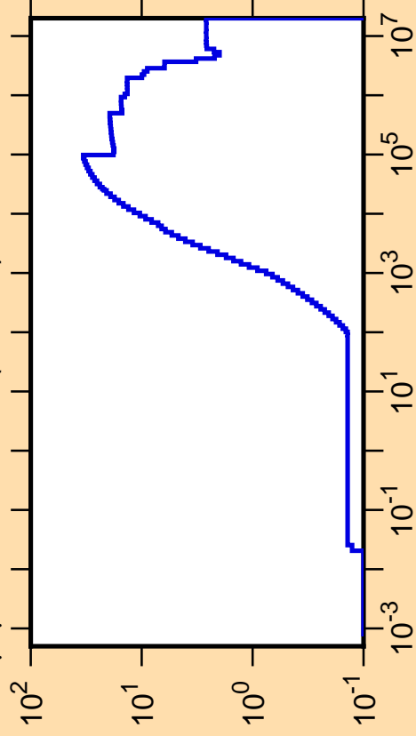
\Delta\mu/\mu vs. E for ^{78}\text{Kr}(\text{mt251})
