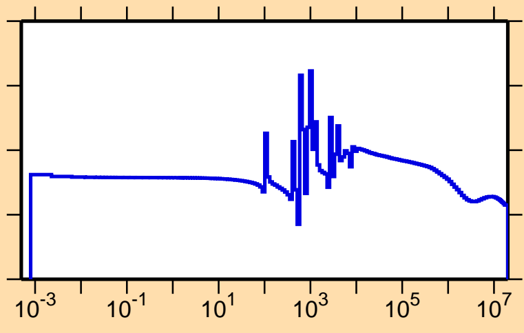
\sigma vs. E for ^{78}\text{Kr}(n,\text{el.})
