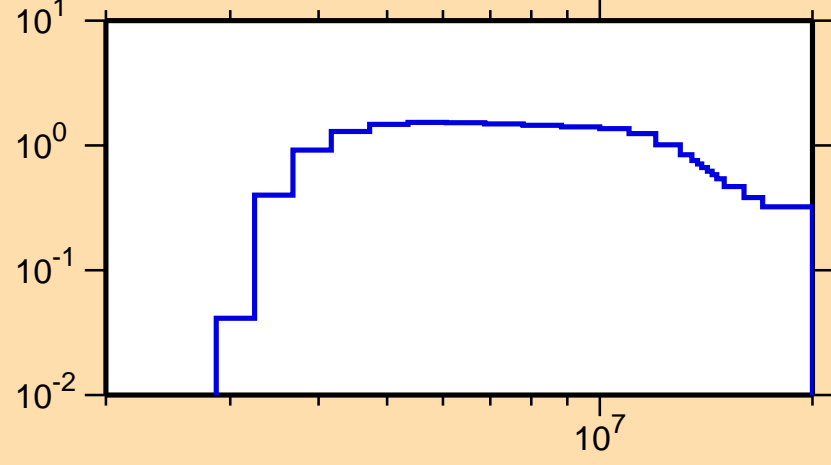
\sigma vs. E for ^{78}\text{Kr}(n,n\text{cont.})
