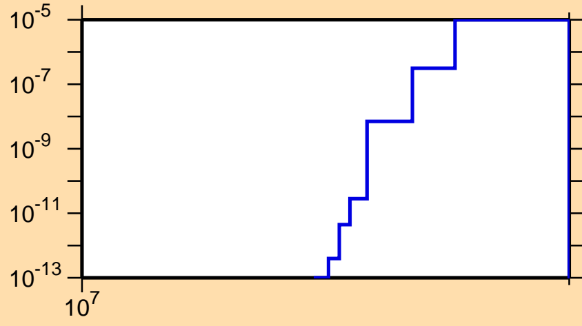
\sigma vs. E for ^{78}\text{Kr}(n,pd)
