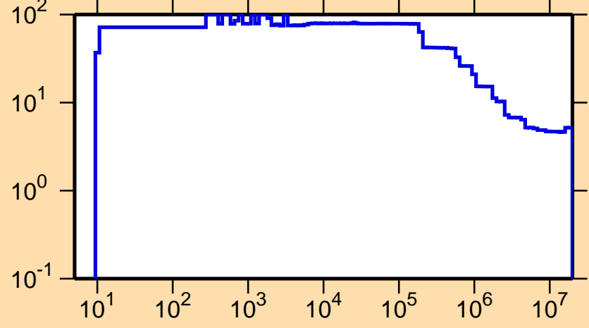
\Delta\sigma/\sigma vs. E for ^{78}\text{Kr}(n,\text{nonel.})
