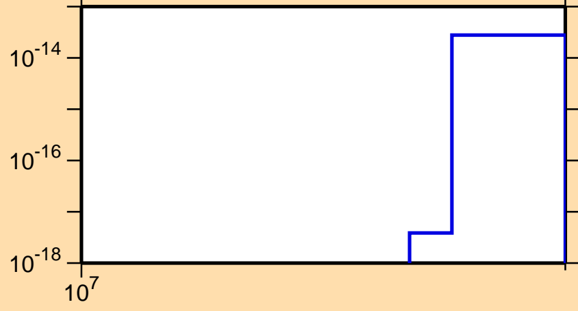
\sigma vs. E for ^{78}\text{Kr}(n,\text{pt})
