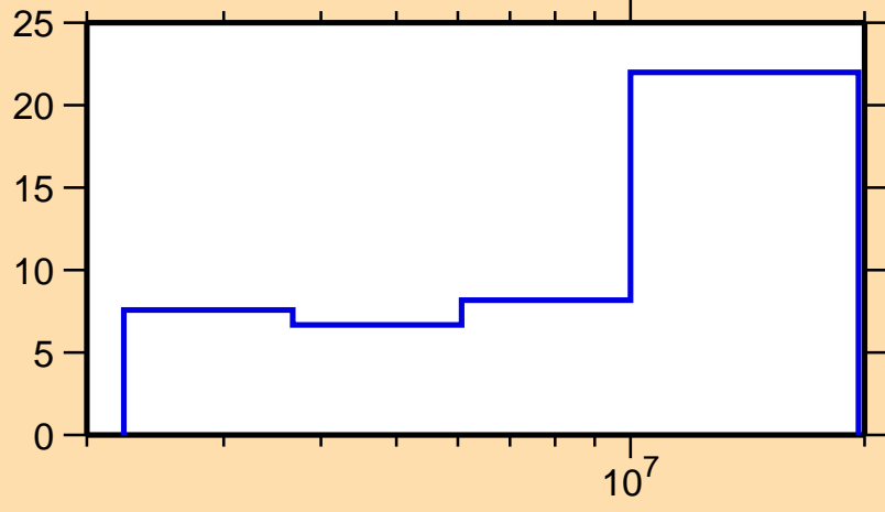
\Delta\sigma/\sigma vs. E for ^{78}\text{Kr}(n,inel.)
