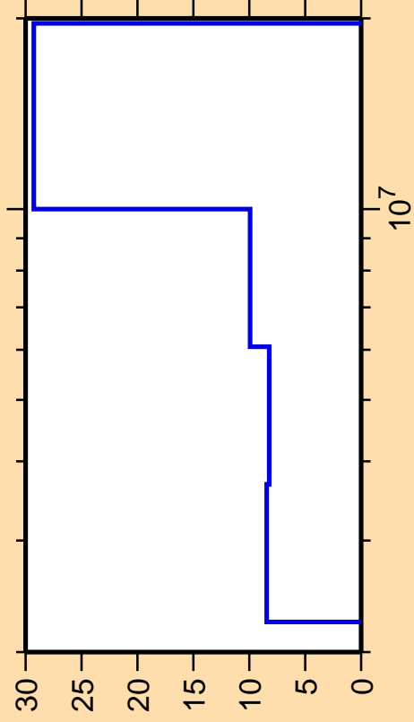
\Delta\sigma/\sigma vs. E for ^{78}\text{Kr}(n,ncont.)
