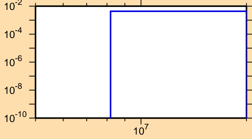
\sigma vs. E for ^{78}\text{Kr}(n,\alpha)
