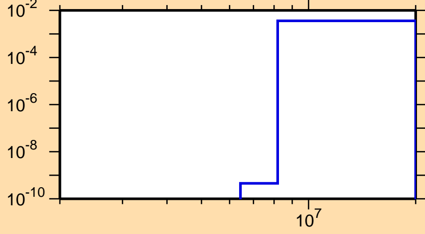
\sigma vs. E for ^{78}\text{Kr}(n,d)
