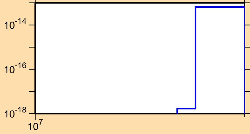
\sigma vs. E for ^{79}\text{Kr}(\text{mt117})
