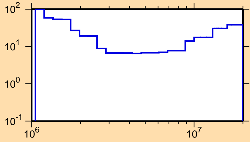
\Delta\sigma/\sigma vs. E for ^{79}\text{Kr}(n,ncont.)
