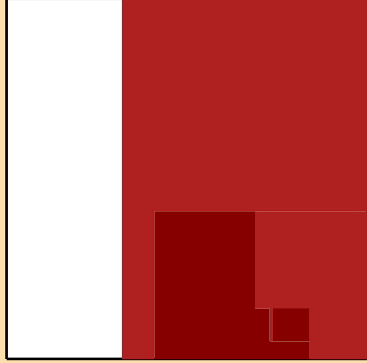
\Delta\sigma/\sigma vs. E for ^{79}\text{Kr}(n,2n)
