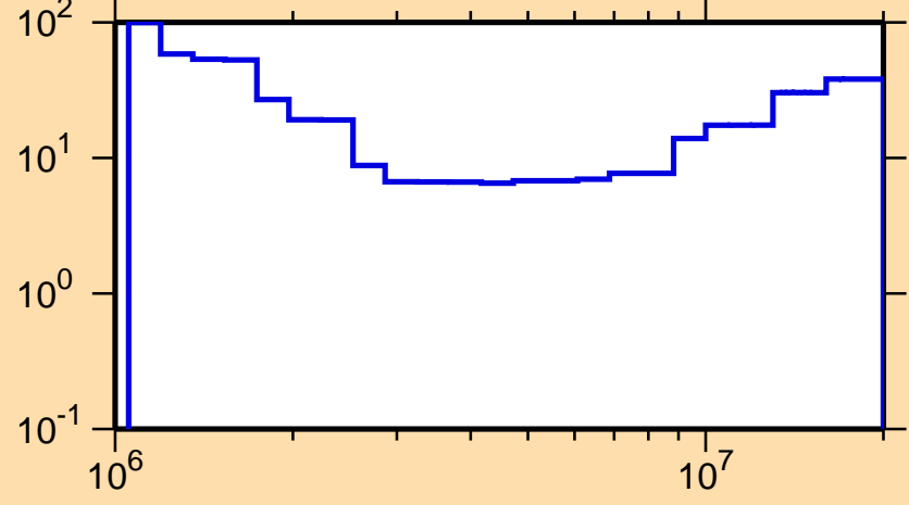
\Delta\sigma/\sigma vs. E for ^{79}\text{Kr}(n,n\text{cont.})
