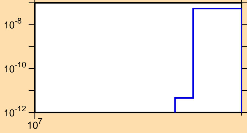
\sigma vs. E for ^{79}\text{Kr}(n,2n\alpha)
