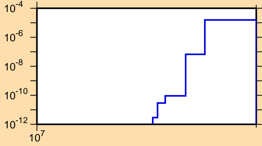
\sigma vs. E for ^{79}\text{Kr}(n,nd)
