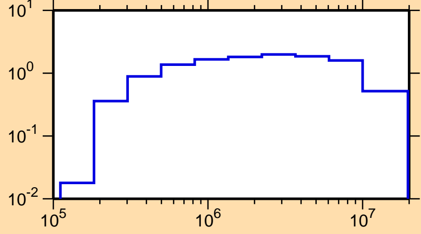
\sigma vs. E for ^{79}\text{Kr}(n,\text{inel.})
