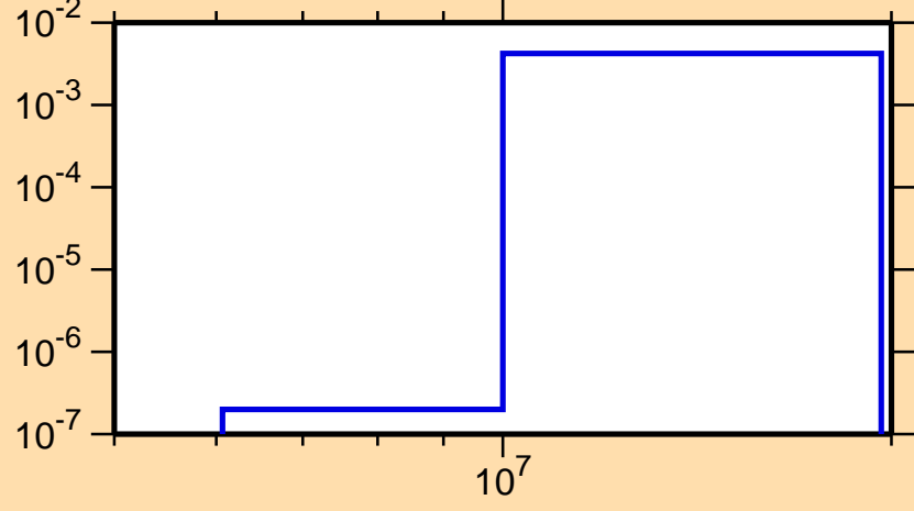
\sigma vs. E for ^{79}\text{Kr}(n,d)
