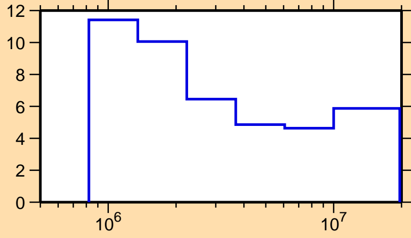
\Delta\sigma/\sigma vs. E for ^{79}\text{Kr}(n,n\text{onel.})
