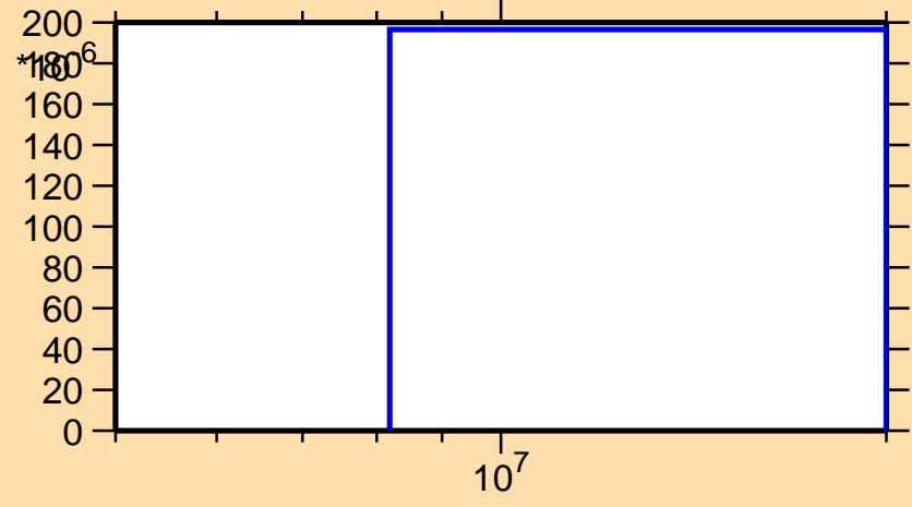
\sigma vs. E for ^{79}\text{Kr}(n,t)
