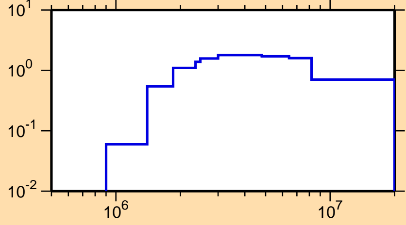
\sigma vs. E for ^{79}\text{Kr}(n,n\text{cont.})
