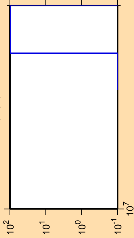
\Delta\sigma/\sigma vs. E for ^{81}\text{Kr}(n,pt)
