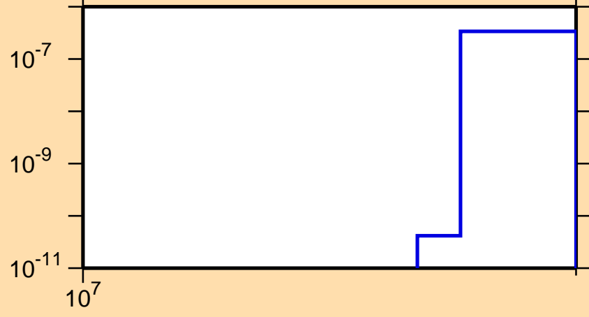
\sigma vs. E for ^{81}\text{Kr}(n,2n\alpha)
