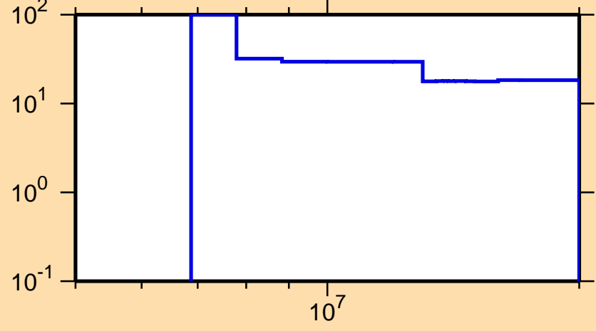
\Delta\sigma/\sigma vs. E for ^{81}\text{Kr}(n,2n)
