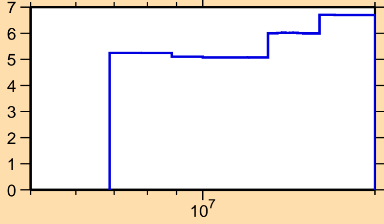
\Delta\sigma/\sigma vs. E for ^{81}\text{Kr}(n,\text{nonel.})
