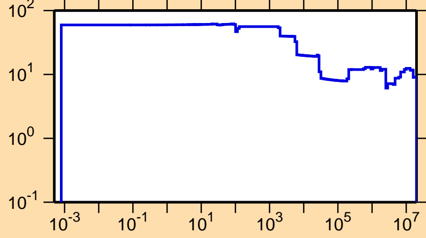
\Delta\sigma/\sigma vs. E for ^{81}\text{Kr}(n,\text{el.})
