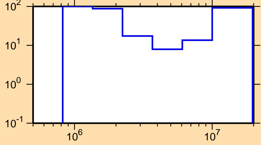
\Delta\sigma/\sigma vs. E for ^{81}\text{Kr}(n,n\text{cont.})
