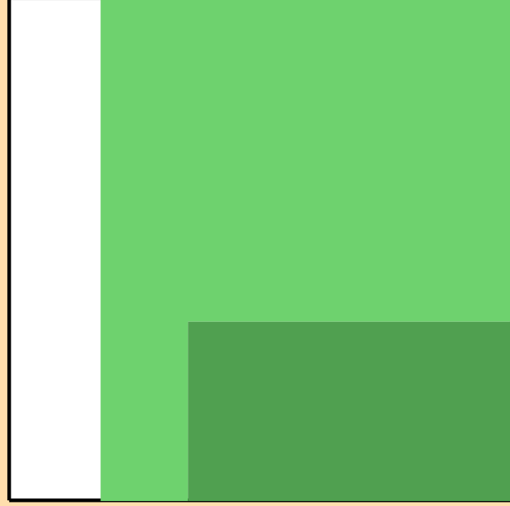
\Delta\sigma/\sigma vs. E for ^{81}\text{Kr}(n,2n)
