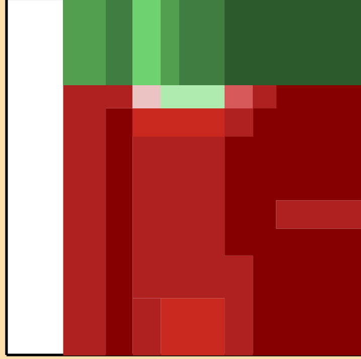
\Delta\sigma/\sigma vs. E for ^{81}\text{Kr}(n,n\text{cont.})
