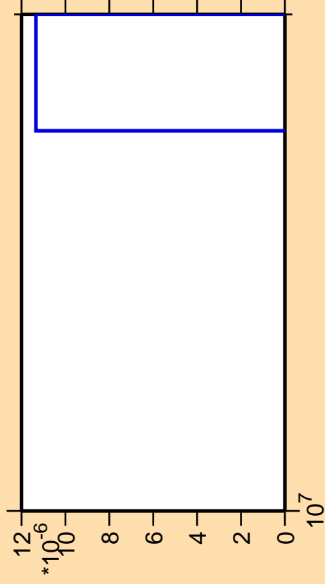
\Delta\sigma/\sigma vs. E for ^{82}\text{Kr}(n,nt)
