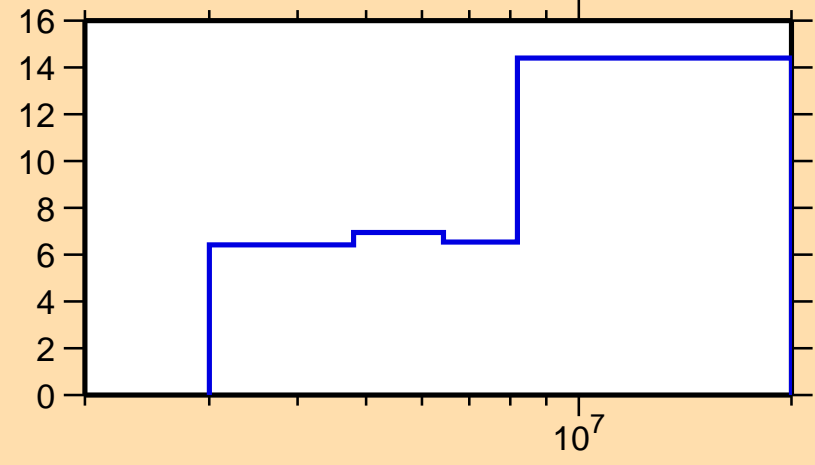
\Delta\sigma/\sigma vs. E for ^{82}\text{Kr}(n,inel.)
