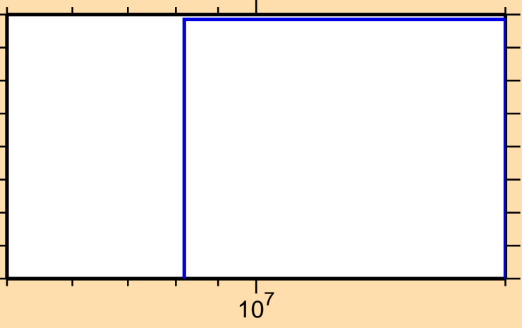
\sigma vs. E for ^{82}\text{Kr}(n,t)
