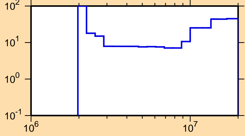
\Delta\sigma/\sigma vs. E for ^{83}\text{Kr}(n,n\text{cont.})
