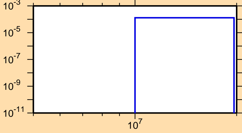
\sigma vs. E for ^{83}\text{Kr}(n,\alpha)
