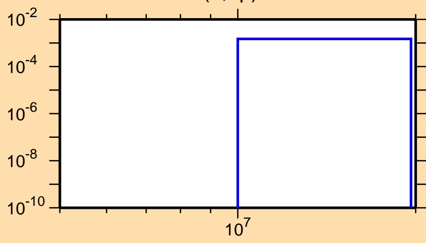
\sigma vs. E for ^{83}\text{Kr}(n,np)
