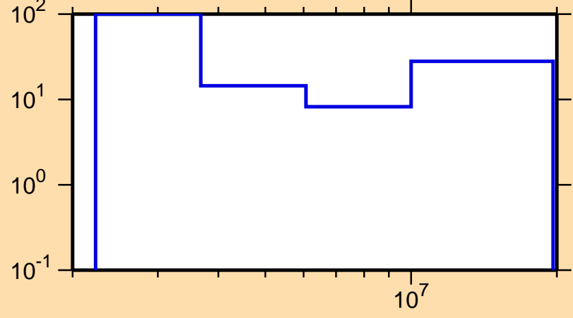
\Delta\sigma/\sigma vs. E for ^{84}\text{Kr}(n,n\text{cont.})
