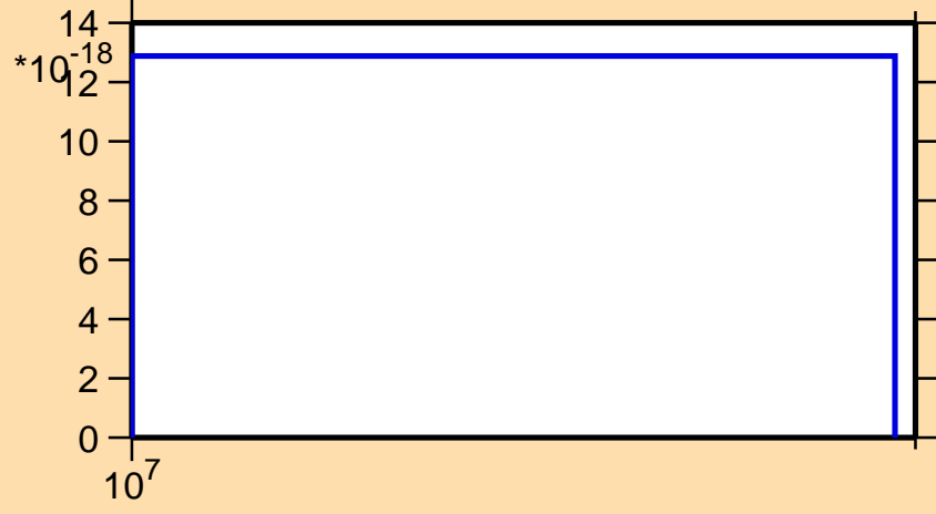
\sigma vs. E for ^{84}\text{Kr}(n,p\alpha)
