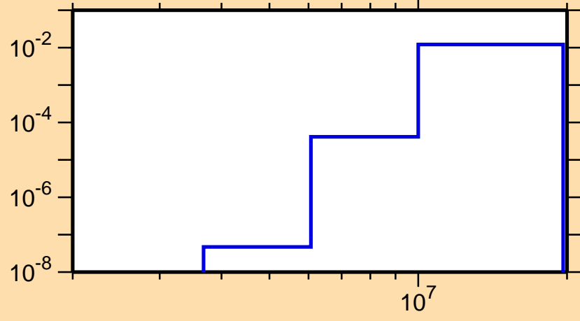
\sigma vs. E for ^{84}\text{Kr}(n,p)
