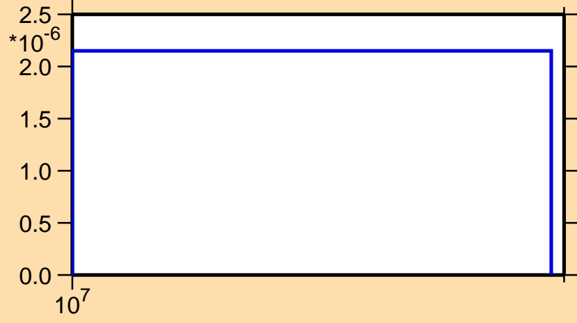
\sigma vs. E for ^{84}\text{Kr}(n,3n)
