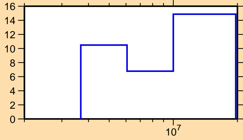
\Delta\sigma/\sigma vs. E for ^{84}\text{Kr}(n,el.)
