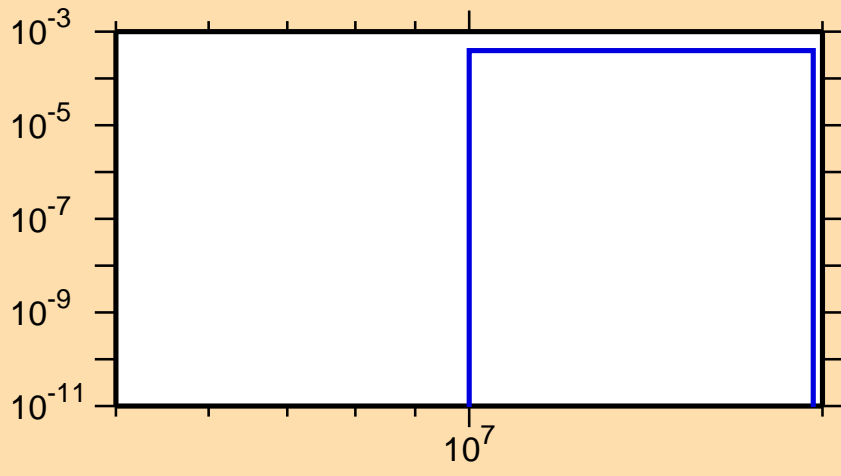
\sigma vs. E for ^{84}\text{Kr}(n,d)
