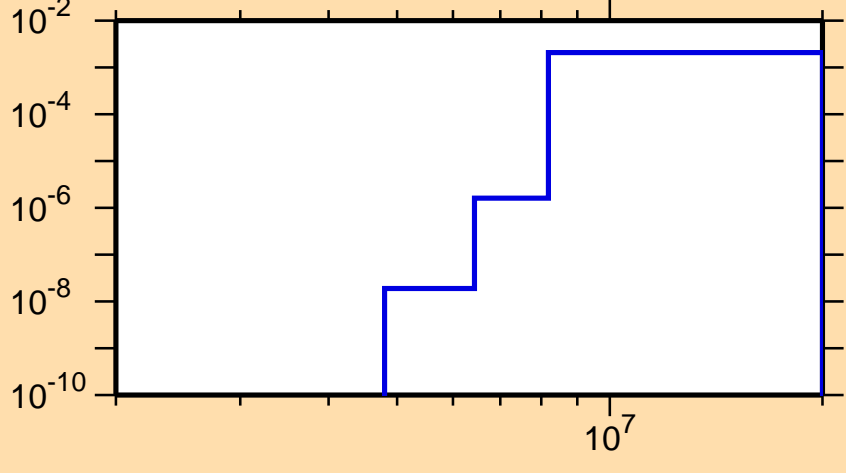
\sigma vs. E for ^{84}\text{Kr}(n,\alpha)
