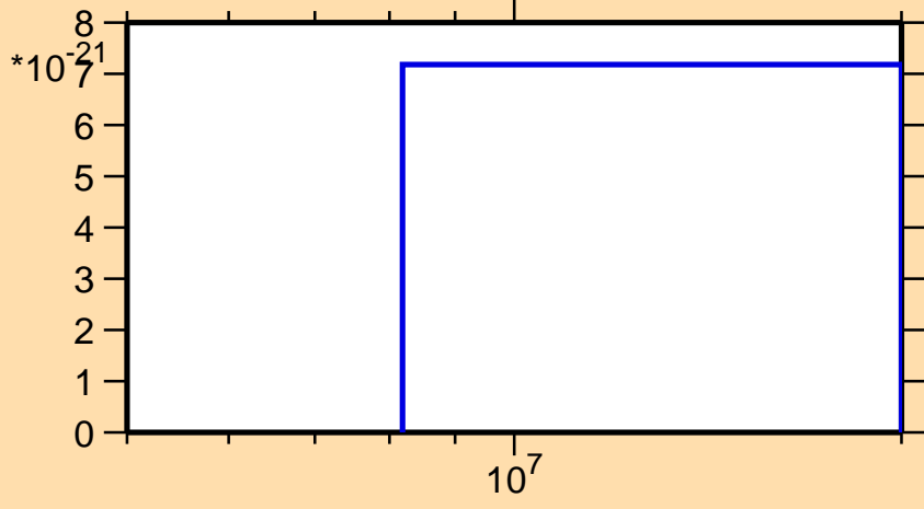
\sigma vs. E for ^{84}\text{Kr}(n,nt)
