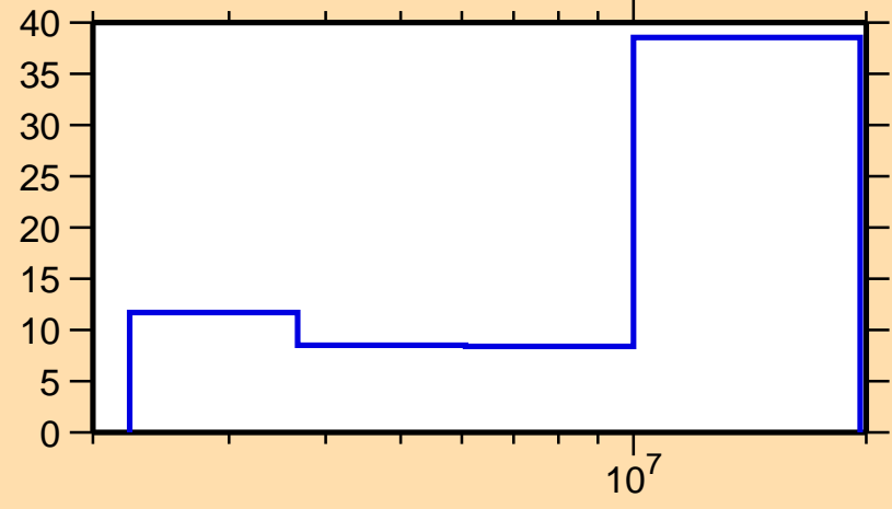
\Delta\sigma/\sigma vs. E for ^{85}\text{Kr}(n,n\text{cont.})
