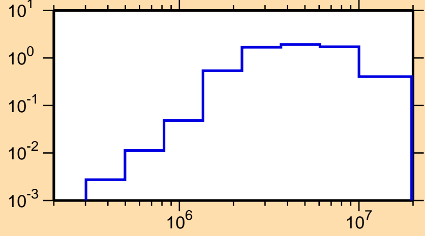
\sigma vs. E for ^{85}\text{Kr}(n,\text{inel.})
