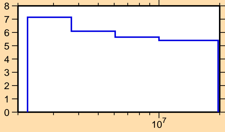
\Delta\sigma/\sigma vs. E for ^{85}\text{Kr}(n,n\text{onel.})
