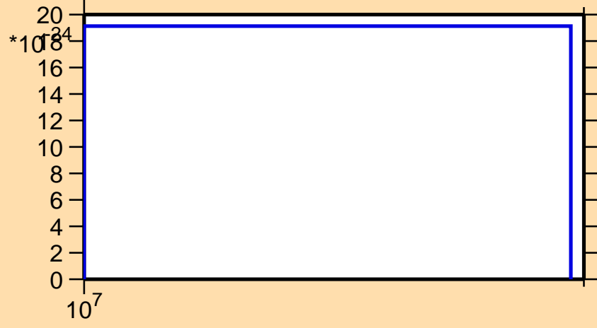
\sigma vs. E for ^{85}\text{Kr}(n,\text{pt})
