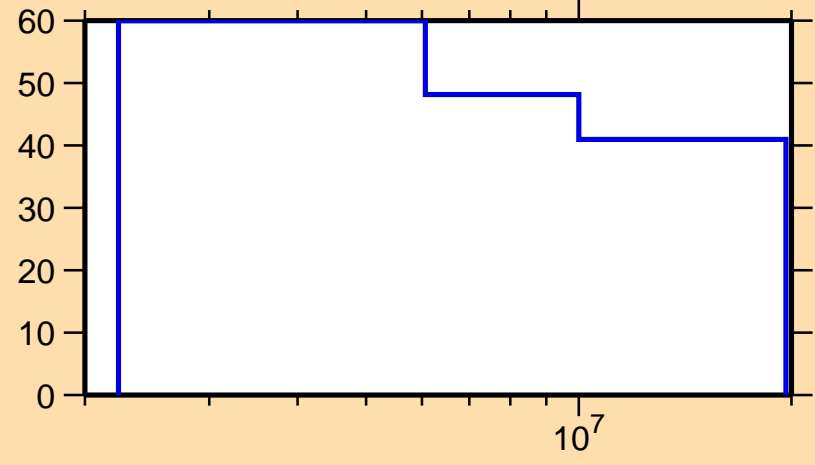
\Delta\sigma/\sigma vs. E for ^{85}\text{Kr}(n,p)
