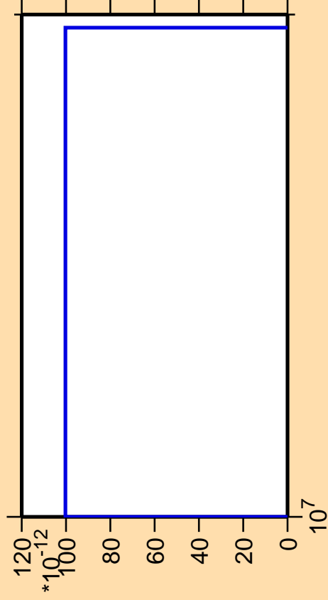
\Delta\sigma/\sigma vs. E for ^{85}\text{Kr}(n,\text{pt})
