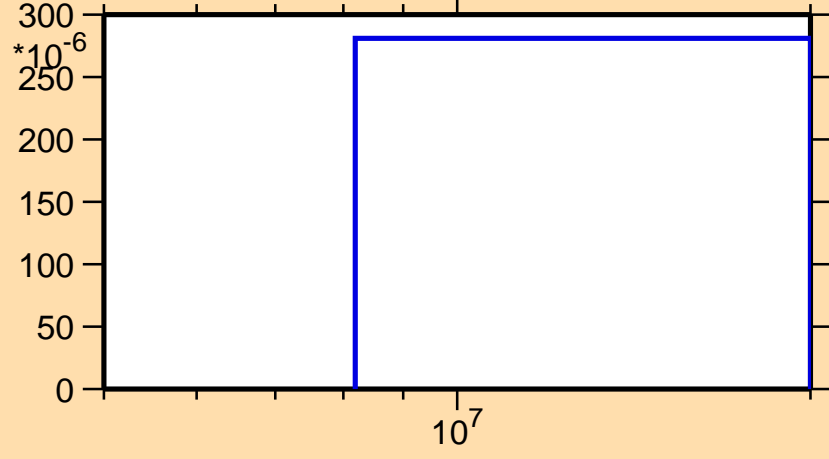
\sigma vs. E for ^{85}\text{Kr}(n,d)
