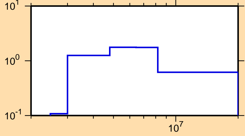
\sigma vs. E for ^{85}\text{Kr}(n,n\text{cont.})
