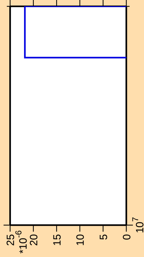
\Delta\sigma/\sigma vs. E for ^{85}\text{Kr}(\text{mt } 34)
