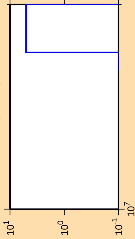
\Delta\sigma/\sigma vs. E for ^{85}\text{Kr}(n,\text{He}3)
