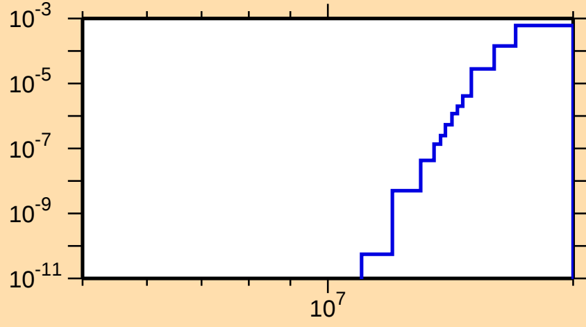
\sigma vs. E for ^{85}\text{Kr}(n,\alpha)
