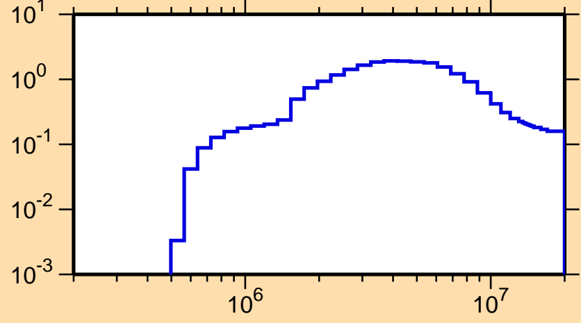
\sigma vs. E for ^{87}\text{Kr}(n,\text{inel.})
