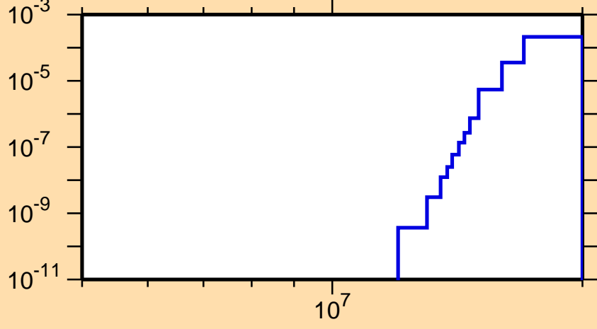
\sigma vs. E for ^{87}\text{Kr}(n,\alpha)
