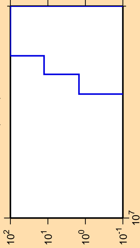
\Delta\sigma/\sigma vs. E for ^{87}\text{Kr}(n,nd)
