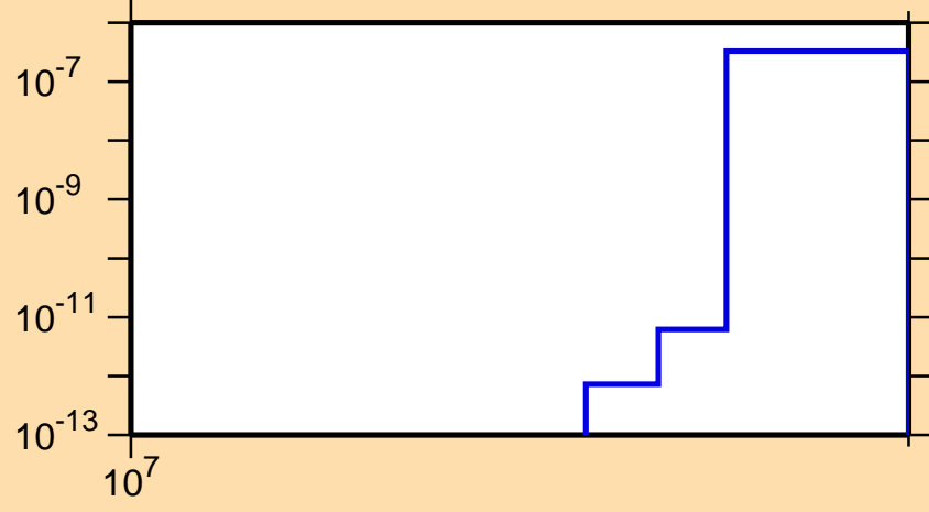
\sigma vs. E for ^{87}\text{Kr}(n,nd)
