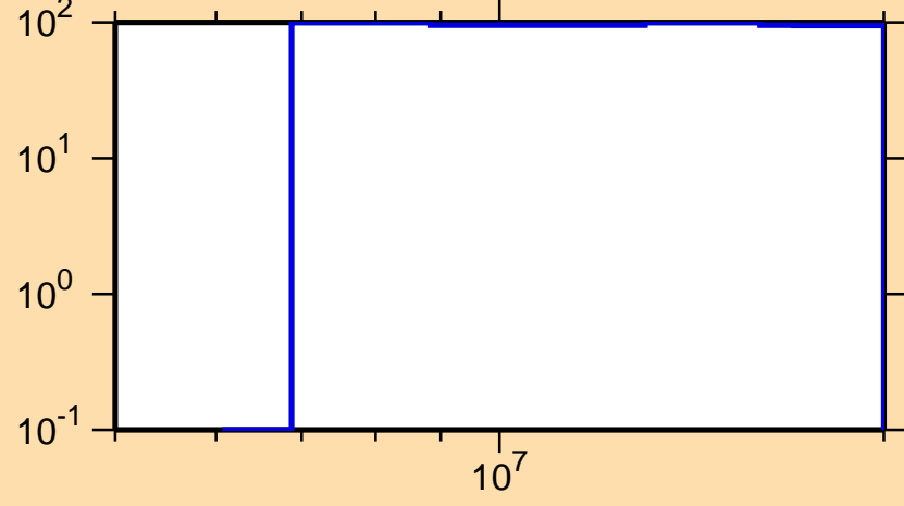
\Delta\sigma/\sigma vs. E for ^{87}\text{Kr}(n,p)
