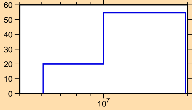
\Delta\sigma/\sigma vs. E for ^{87}\text{Kr}(n,ncont.)
