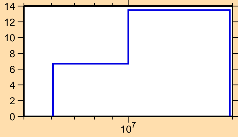
\Delta\sigma/\sigma vs. E for ^{87}\text{Kr}(n,el.)
