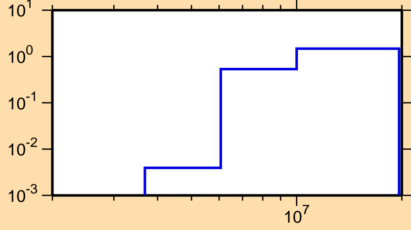
\sigma vs. E for ^{87}\text{Kr}(n,2n)
