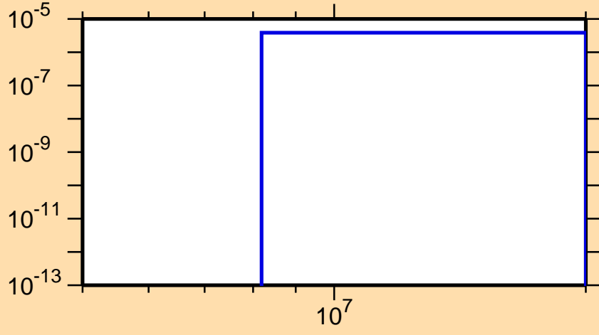
\sigma vs. E for ^{87}\text{Kr}(n,\alpha)
