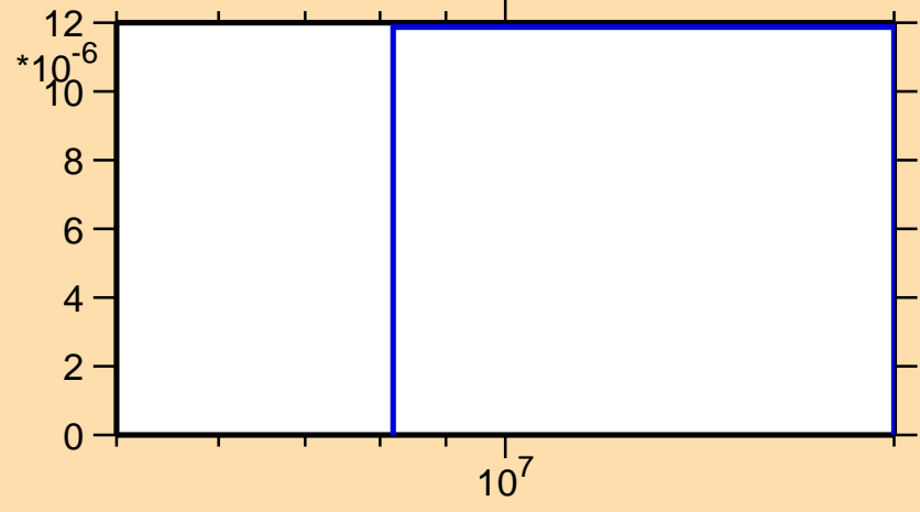
\sigma vs. E for ^{87}\text{Kr}(n,t)
