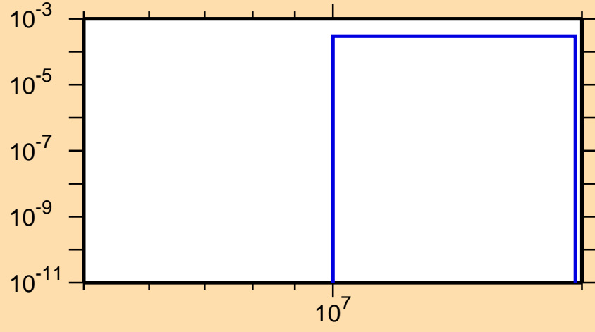
\sigma vs. E for ^{88}\text{Kr}(n,p)
