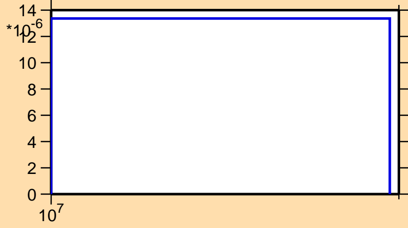
\sigma vs. E for ^{88}\text{Kr}(n,d)
