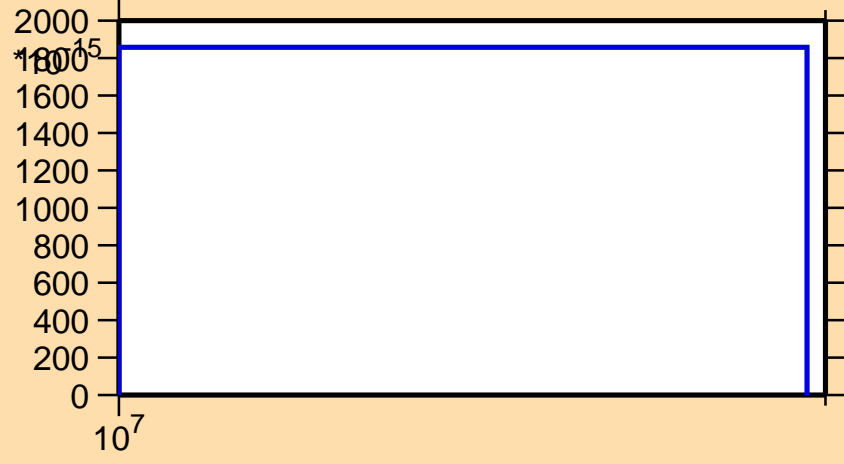
\sigma vs. E for ^{88}\text{Kr}(n,\text{nd})
