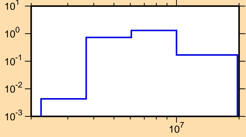
\sigma vs. E for ^{88}\text{Kr}(n,n\text{cont.})
