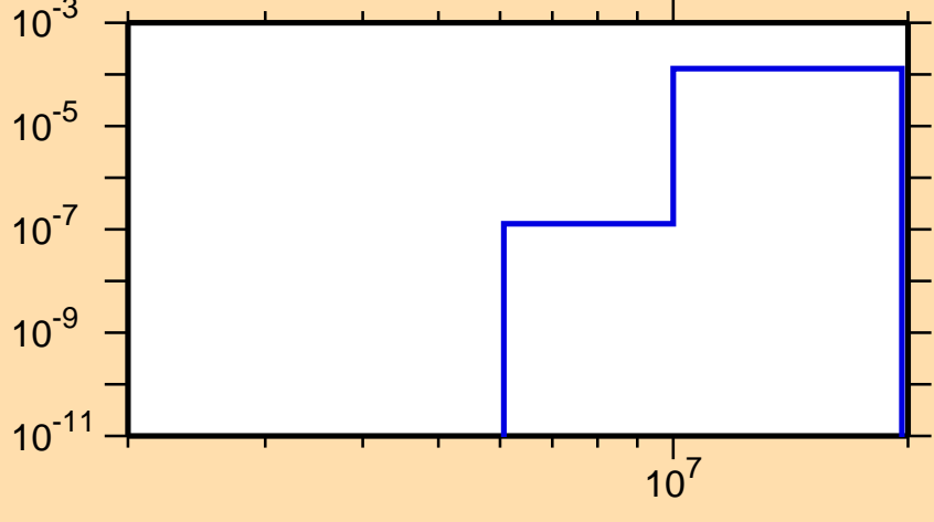
\sigma vs. E for ^{88}\text{Kr}(n,\alpha)
