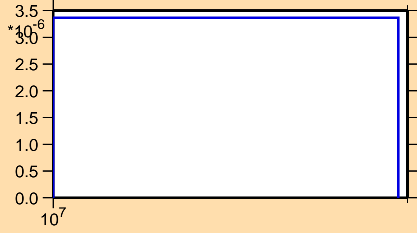
\sigma vs. E for ^{88}\text{Kr}(n,t)
