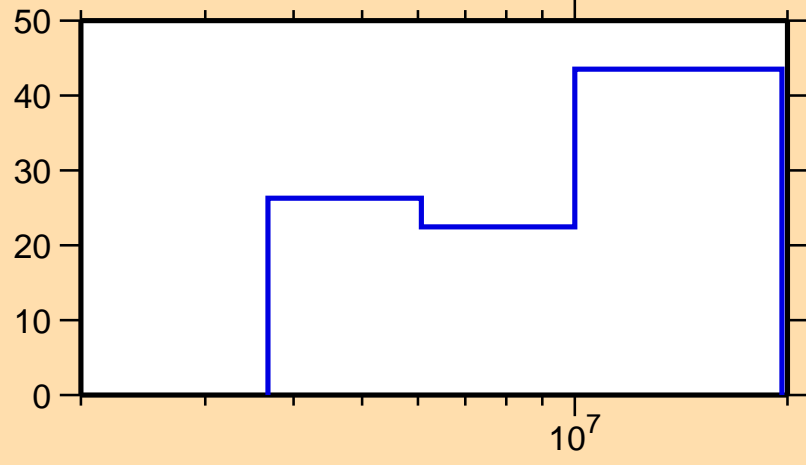
\Delta\sigma/\sigma vs. E for ^{88}\text{Kr}(n,n\text{cont.})
