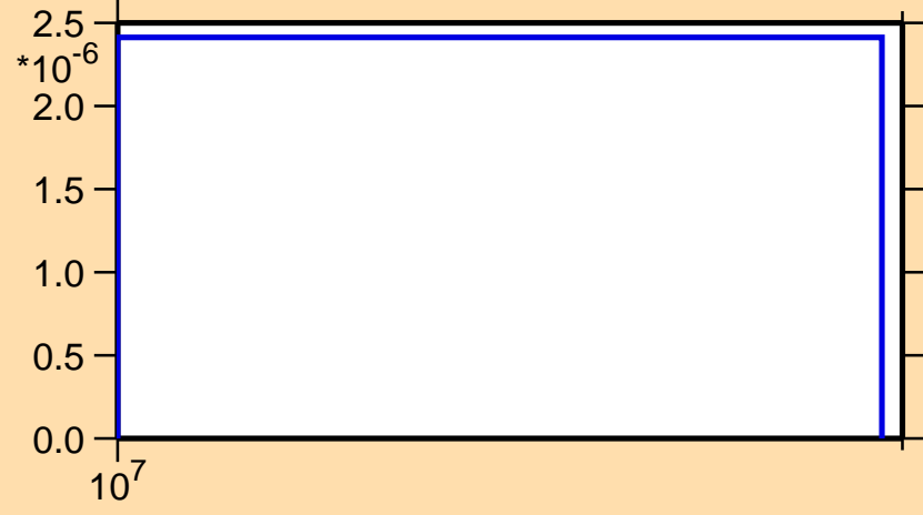
\sigma vs. E for ^{88}\text{Kr}(n,np)
