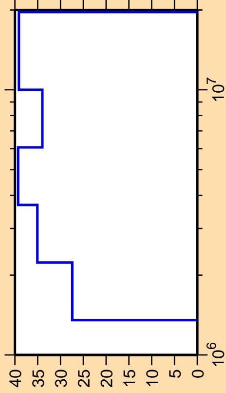
\Delta\sigma/\sigma vs. E for ^{88}\text{Kr}(n,n_3)
