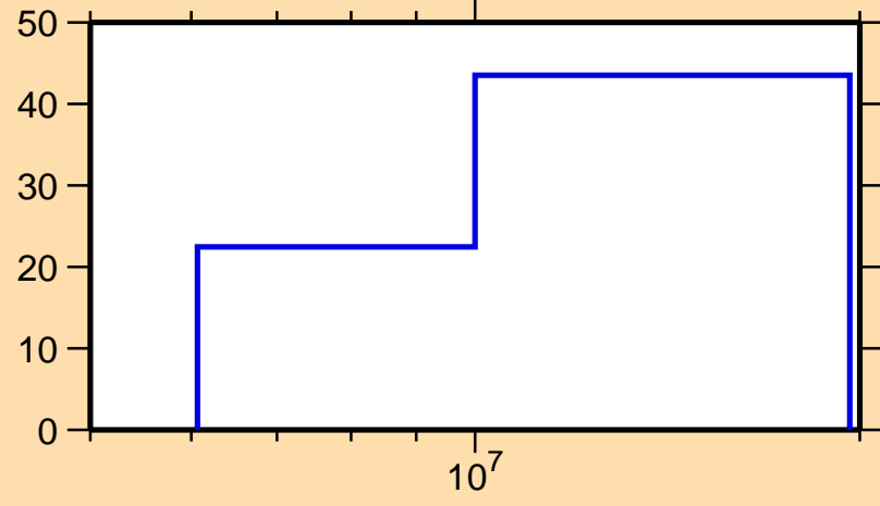
\Delta\sigma/\sigma vs. E for ^{88}\text{Kr}(n,ncont.)
