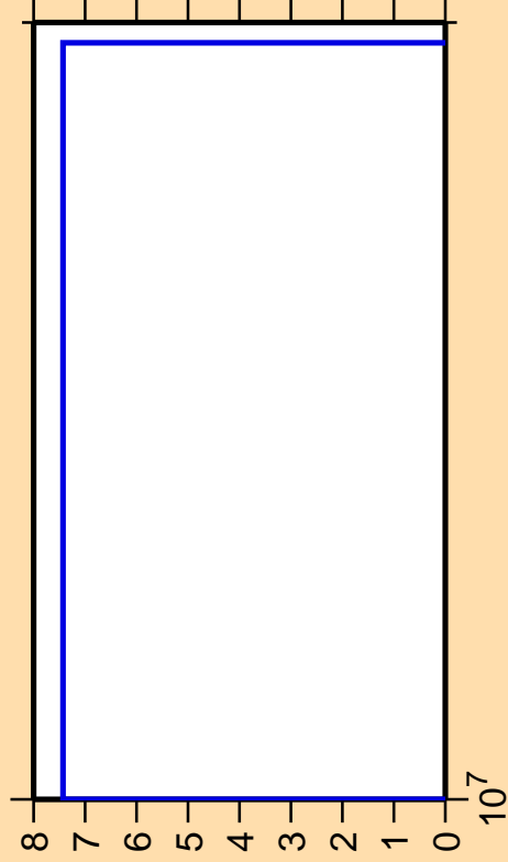
\Delta\sigma/\sigma vs. E for ^{88}\text{Kr}(n,\text{nd})
