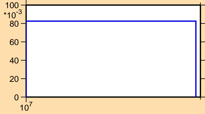
\sigma vs. E for ^{88}\text{Kr}(n,3n)
