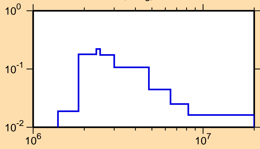
\sigma vs. E for ^{88}\text{Kr}(n,n_3)
