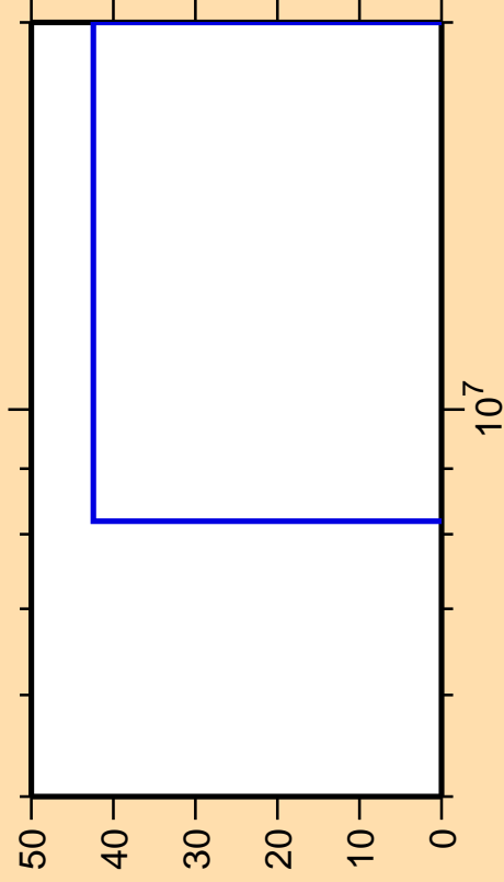
\Delta\sigma/\sigma vs. E for ^{88}\text{Kr}(n,n\alpha)
