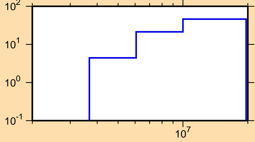
\Delta\sigma/\sigma vs. E for ^{89}\text{Kr}(n,\text{inel.})
