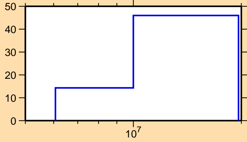
\Delta\sigma/\sigma vs. E for ^{89}\text{Kr}(n,ncont.)
