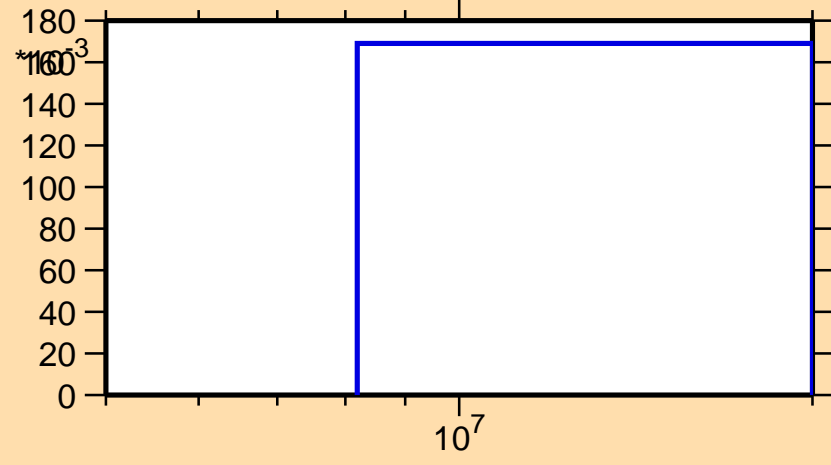
\sigma vs. E for ^{89}\text{Kr}(n,3n)
