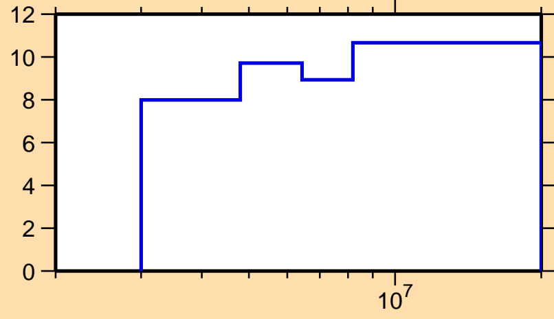
\Delta\sigma/\sigma vs. E for ^{89}\text{Kr}(n,n\text{onel.})
