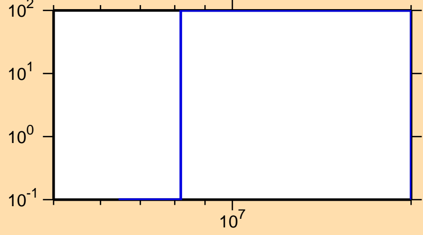
\Delta\sigma/\sigma vs. E for ^{89}\text{Kr}(n,p)
