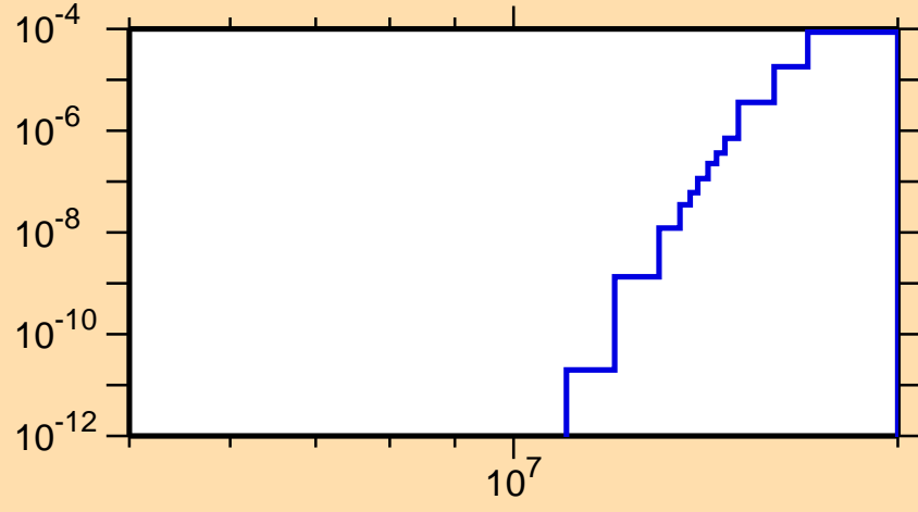
\sigma vs. E for ^{90}\text{Kr}(n,\alpha)
