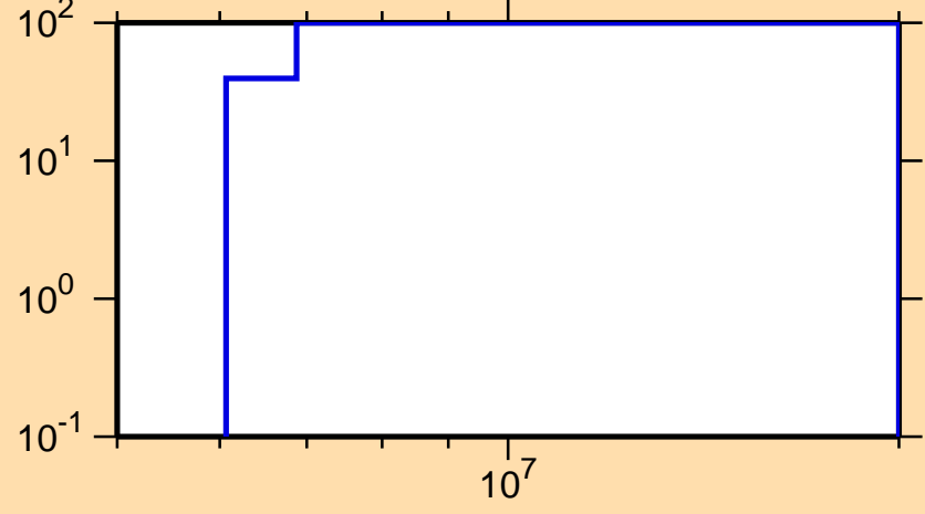
\Delta\sigma/\sigma vs. E for ^{90}\text{Kr}(n,n\text{cont.})
