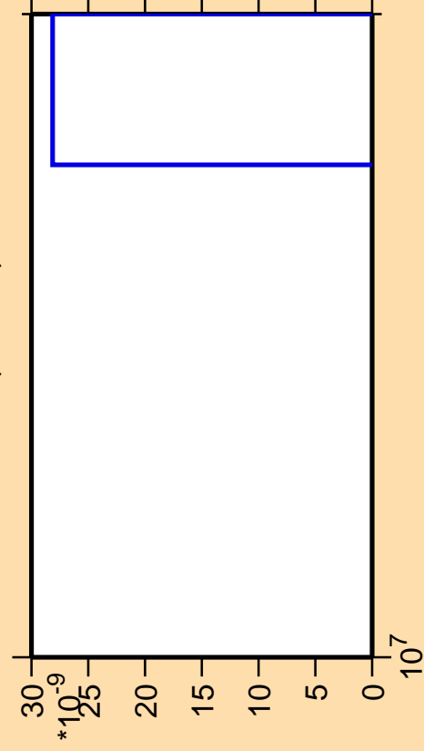
\Delta\sigma/\sigma vs. E for ^{90}\text{Kr}(n,\text{He}3)
