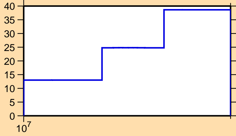
\Delta\sigma/\sigma vs. E for ^{90}\text{Kr}(n,el.)
