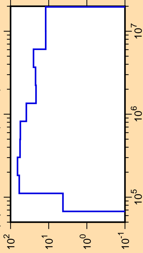
\Delta\mu/\mu vs. E for ^{92}\text{Kr}(\text{mt251})
