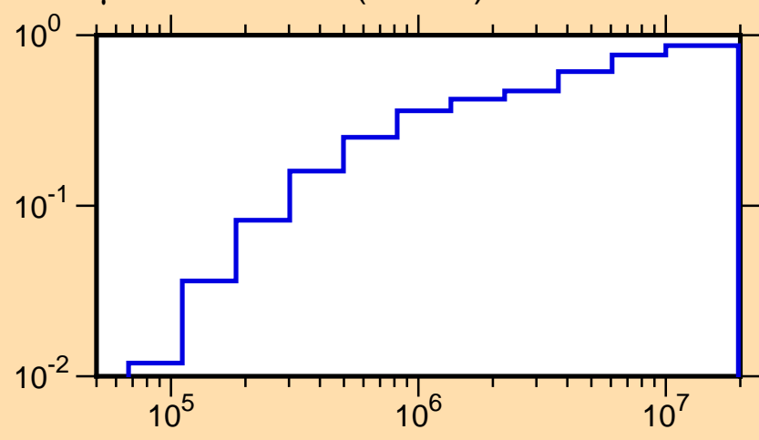
\mu vs. E for ^{92}\text{Kr}(\text{mt251})
