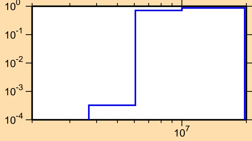
\sigma vs. E for ^{92}\text{Kr}(n,2n)
