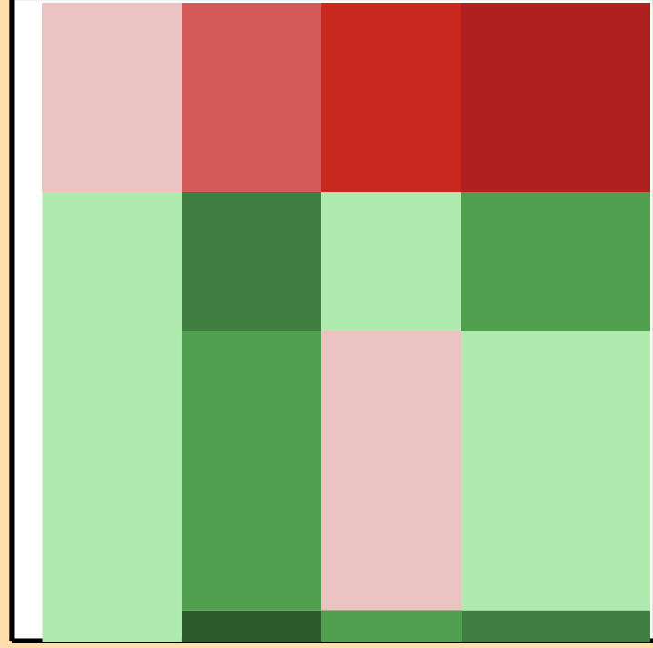
\Delta\sigma/\sigma vs. E for ^{92}\text{Kr}(n,n\text{cont.})
