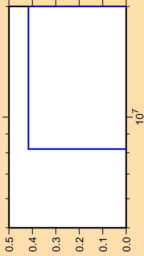
\Delta\sigma/\sigma vs. E for ^{92}\text{Kr}(n,nd)
