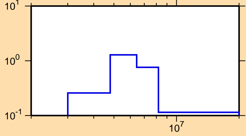
\sigma vs. E for ^{92}\text{Kr}(n,n\text{cont.})
