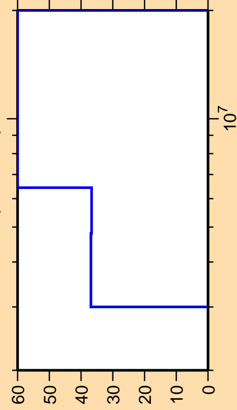
\Delta\sigma/\sigma vs. E for ^{92}\text{Kr}(n,ncont.)
