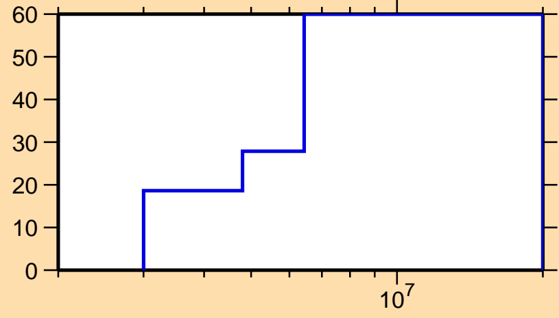
\Delta\sigma/\sigma vs. E for ^{92}\text{Kr}(n,inel.)
