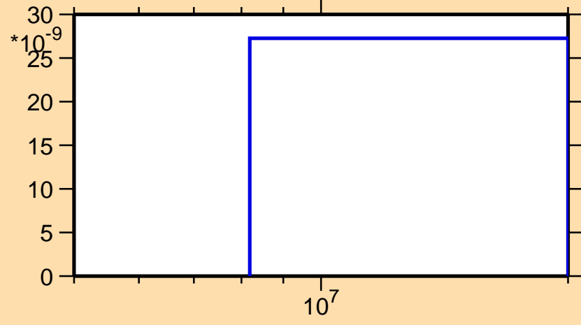
\sigma vs. E for ^{92}\text{Kr}(n,np)
