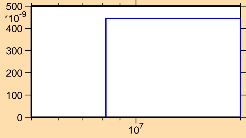
\sigma vs. E for ^{92}\text{Kr}(n,d)
