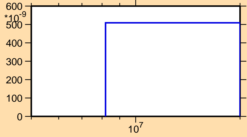
\sigma vs. E for ^{92}\text{Kr}(n,t)
