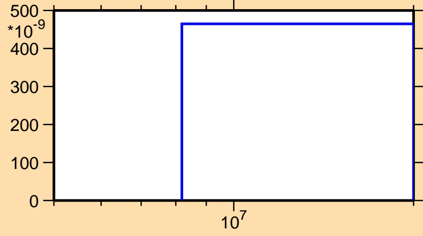
\sigma vs. E for ^{92}\text{Kr}(n,\alpha)
