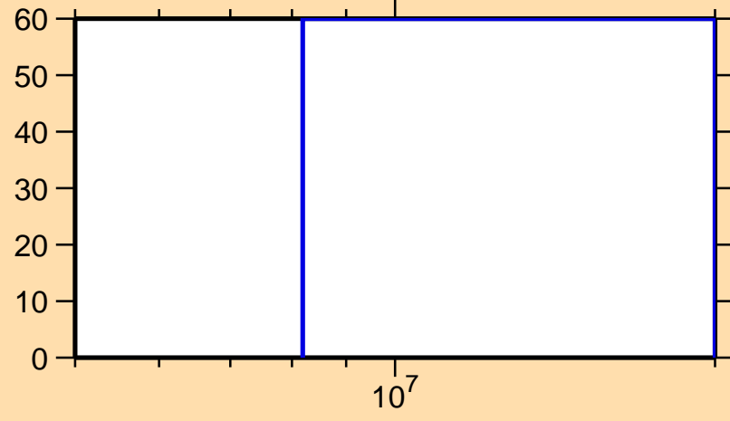
\Delta\sigma/\sigma vs. E for ^{92}\text{Kr}(n,ncont.)
