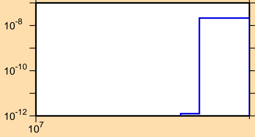
\sigma vs. E for ^{93}\text{Kr}(n,\text{nd})
