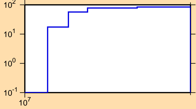
\Delta\sigma/\sigma vs. E for ^{93}\text{Kr}(n,p)
