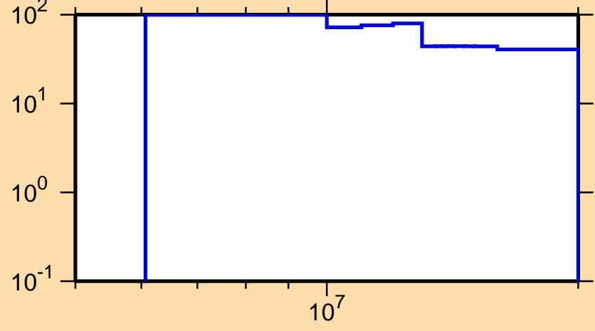
\Delta\sigma/\sigma vs. E for ^{93}\text{Kr}(n,n\text{cont.})
