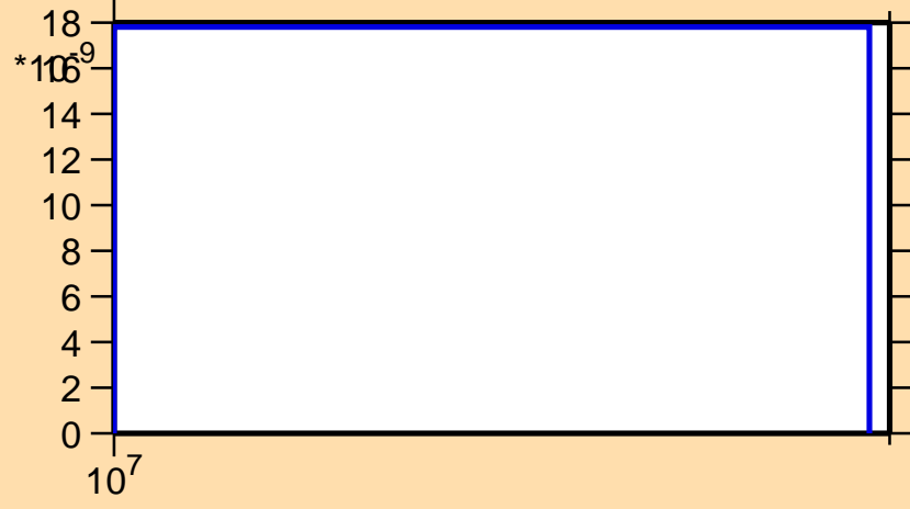
\sigma vs. E for ^{93}\text{Kr}(n,np)
