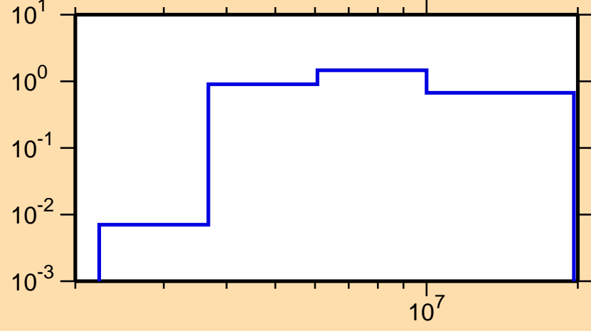
\sigma vs. E for ^{93}\text{Kr}(n,2n)
