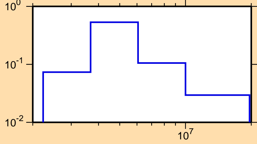
\sigma vs. E for ^{93}\text{Kr}(n,n\text{cont.})
