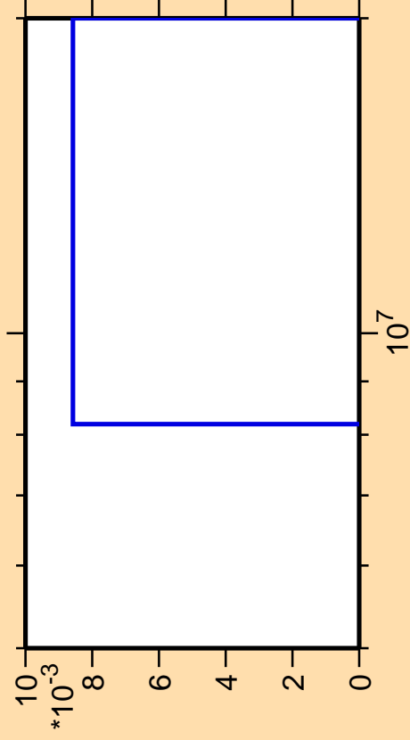
\Delta\sigma/\sigma vs. E for ^{93}\text{Kr}(n,2np)
