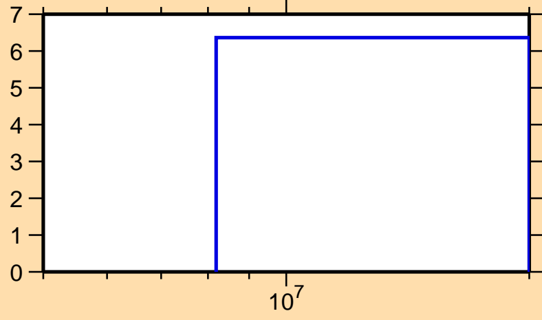
\Delta\sigma/\sigma vs. E for ^{93}\text{Kr}(n,\text{tot.})
