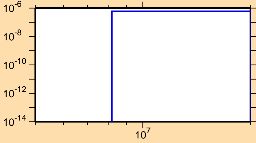
\sigma vs. E for ^{93}\text{Kr}(n,\alpha)
