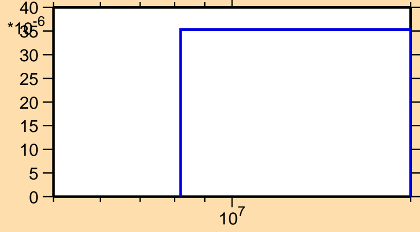
\sigma vs. E for ^{93}\text{Kr}(n,p)
