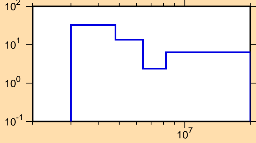
\Delta\sigma/\sigma vs. E for ^{93}\text{Kr}(n,\text{tot.})
