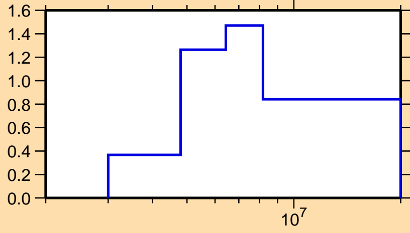
\sigma vs. E for ^{93}\text{Kr}(n,2n)
