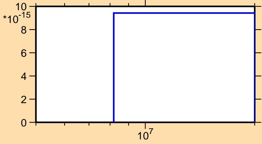
\sigma vs. E for ^{93}\text{Kr}(n,2np)
