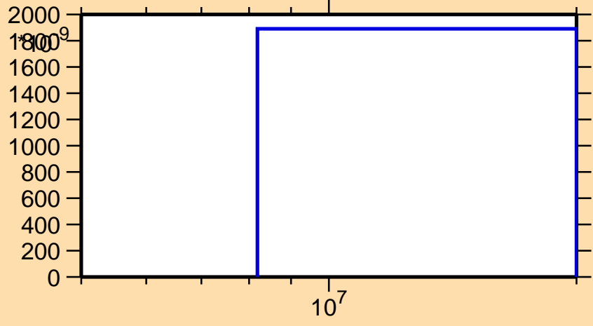
\sigma vs. E for ^{93}\text{Kr}(n,t)
