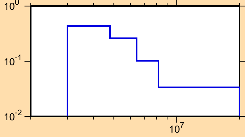
\sigma vs. E for ^{93}\text{Kr}(n,n\text{cont.})
