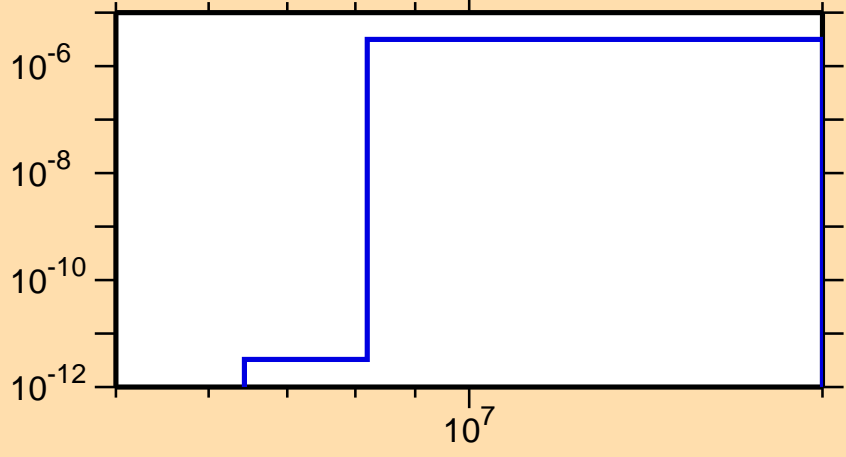
\sigma vs. E for ^{93}\text{Kr}(n,\alpha)
