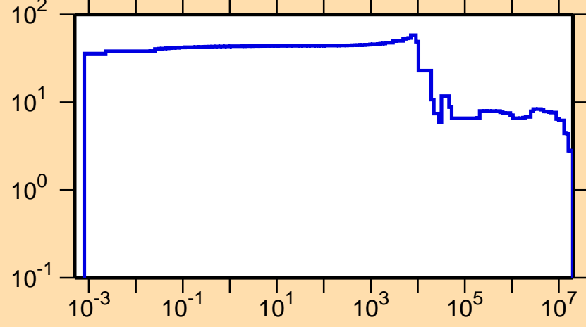
\Delta\sigma/\sigma vs. E for ^{22}\text{Mg}(n,\text{tot.})
