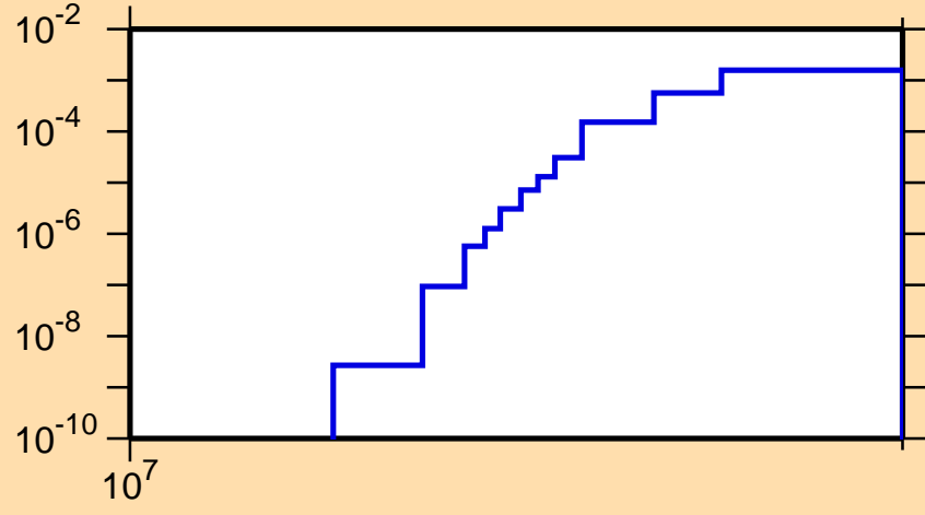
\sigma vs. E for ^{22}\text{Mg}(\text{mt117})
