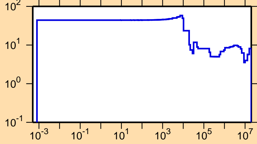
\Delta\sigma/\sigma vs. E for ^{22}\text{Mg}(n,\text{el.})
