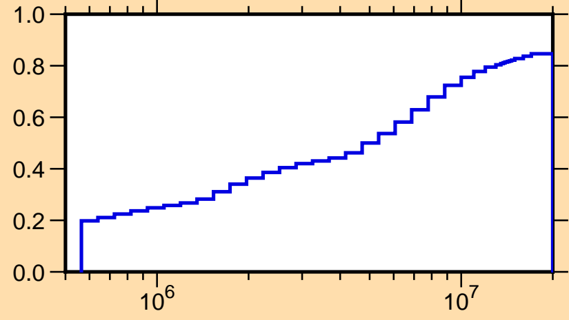
\mu vs. E for ^{24}\text{Mg}(\text{mt251})
