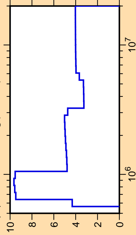
\Delta\mu/\mu vs. E for ^{24}\text{Mg}(\text{mt251})
