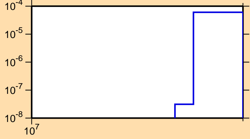
\sigma vs. E for ^{24}\text{Mg}(n,t)
