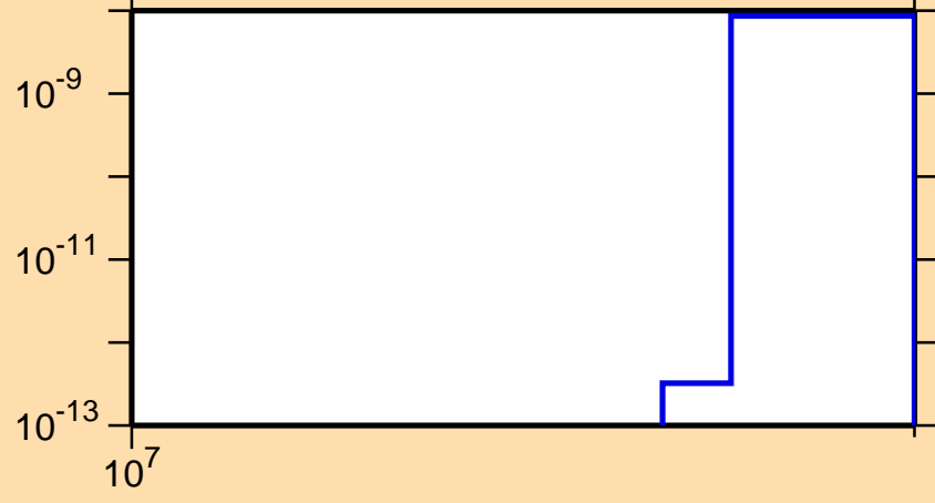
\sigma vs. E for ^{24}\text{Mg}(n,p\alpha)
