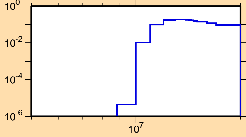
\sigma vs. E for ^{24}\text{Mg}(n,n\text{cont.})
